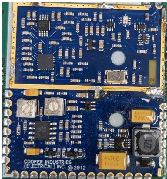
Figure 1 LPT900 board's top view with shield's lid removed.
