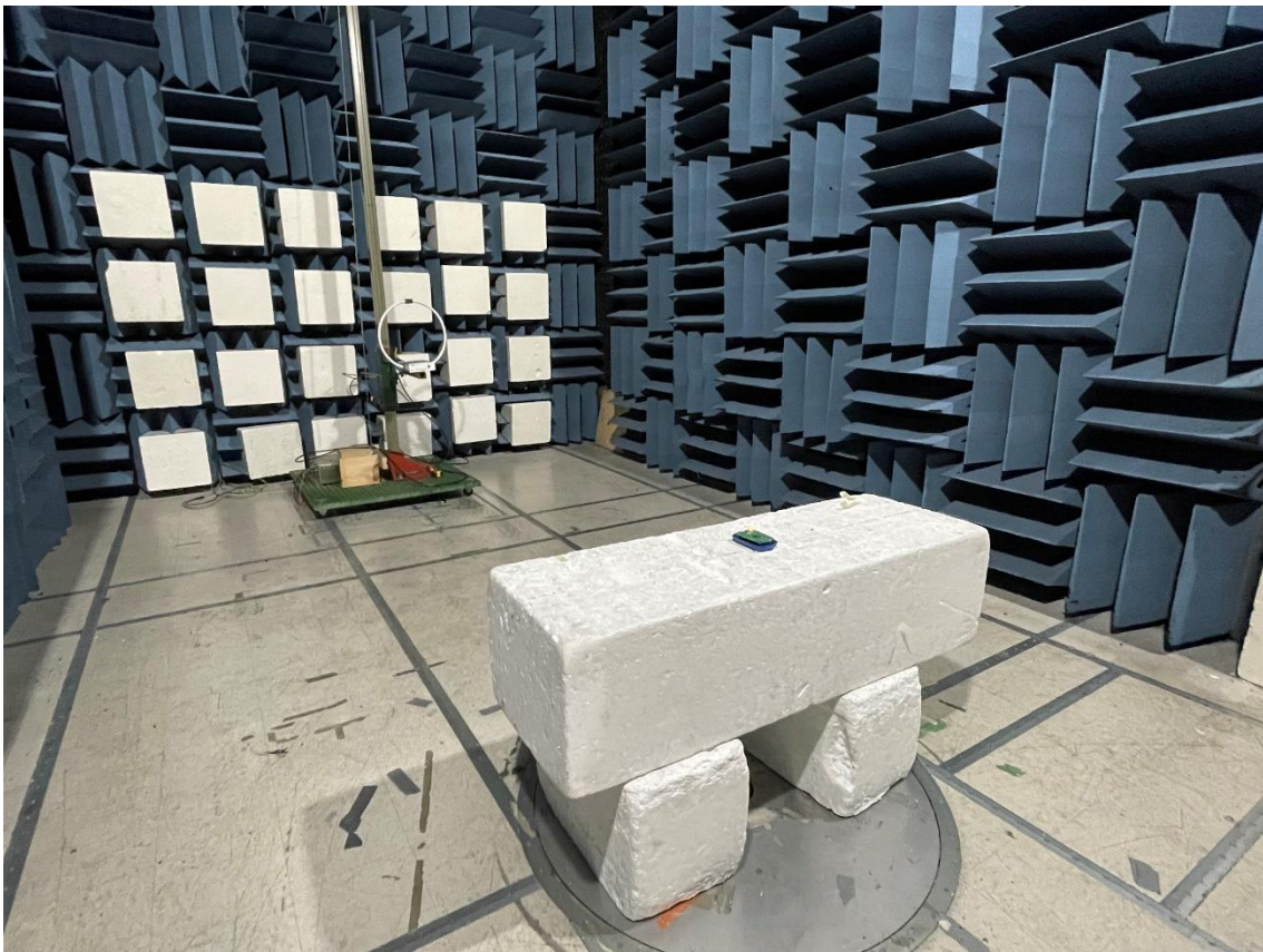
Test setup of radiated emissions below 30 MHz
