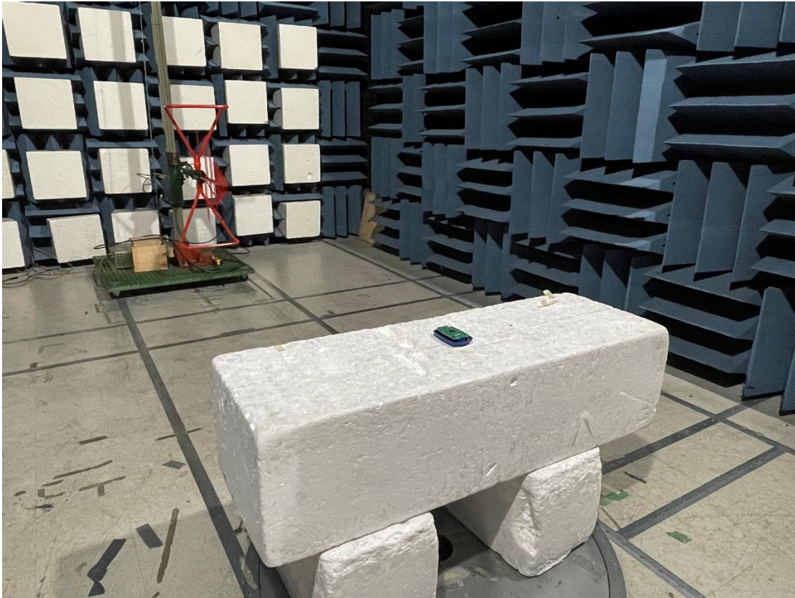
Test setup of radiated emissions between 30 MHz and 1000 MHz
