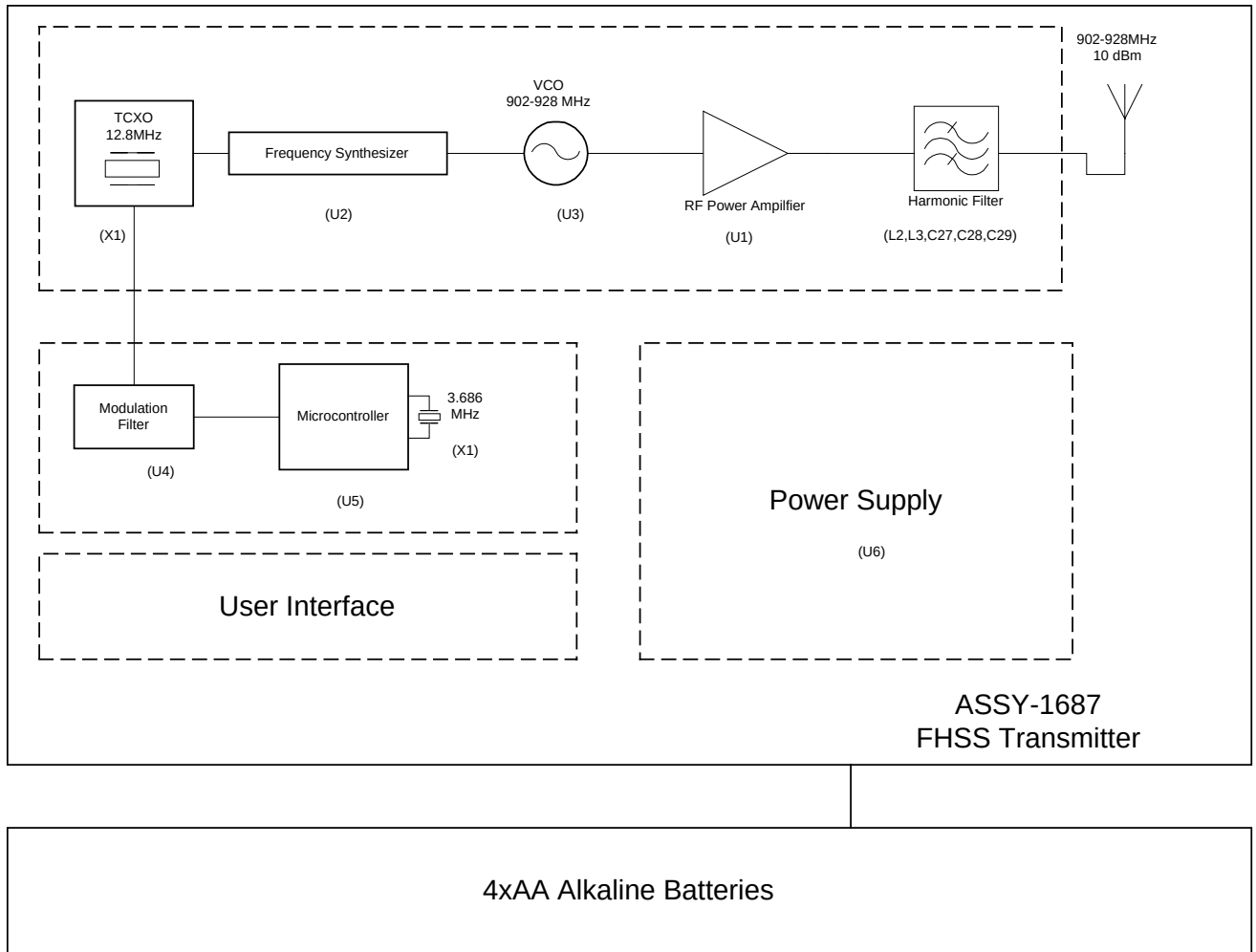
Figure 1. Transmitter System Block Diagram
