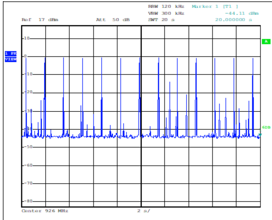
Plot 5: 13 Burst in 20 s
