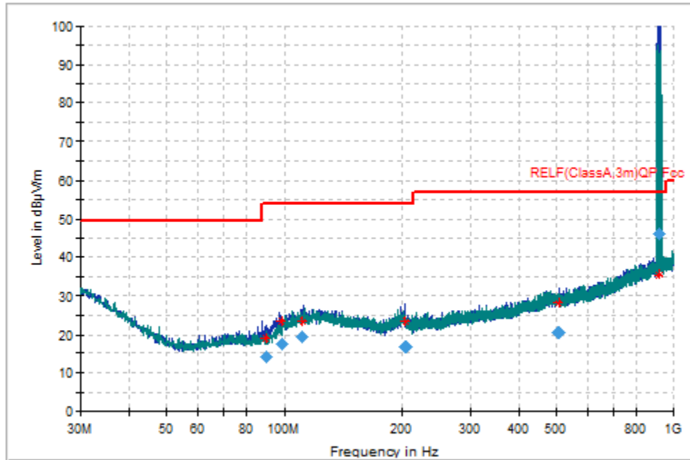
Plot 1: Radiated Emissions at 3m SAC – FCC Part 15/B 15.109; ICES-003, mode #1
