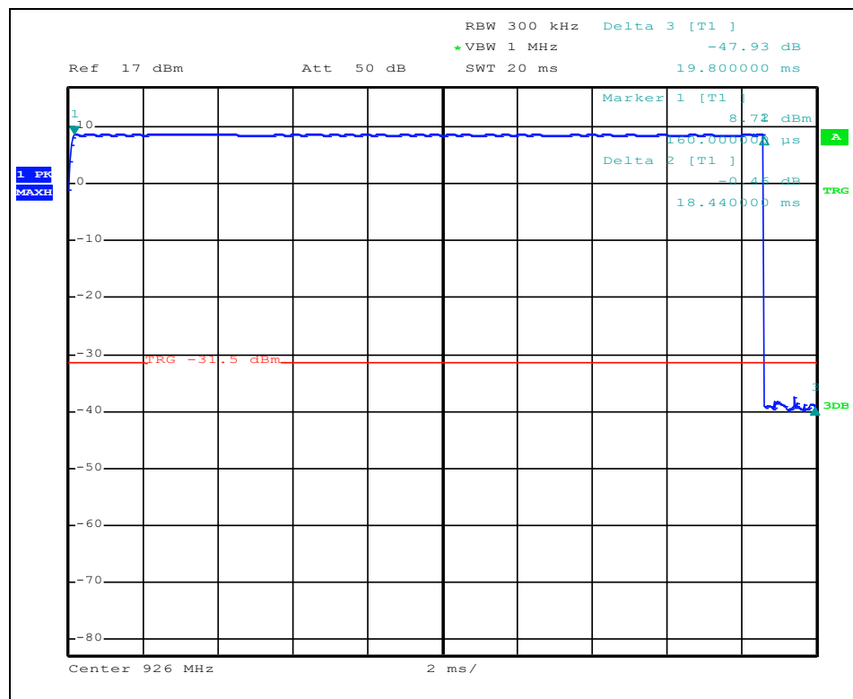
Plot 4: Bursts in 100ms- Dwelling time 18.44 ms
