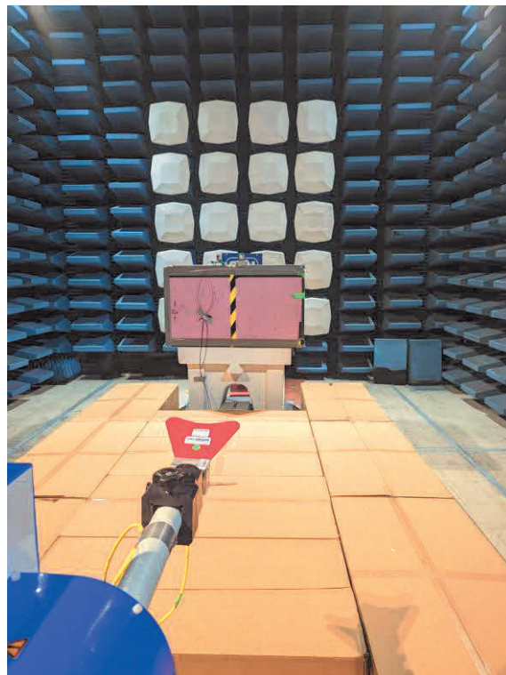
Figure 55: Radiated Emissions Setup: 1 GHz - 18 GHz
