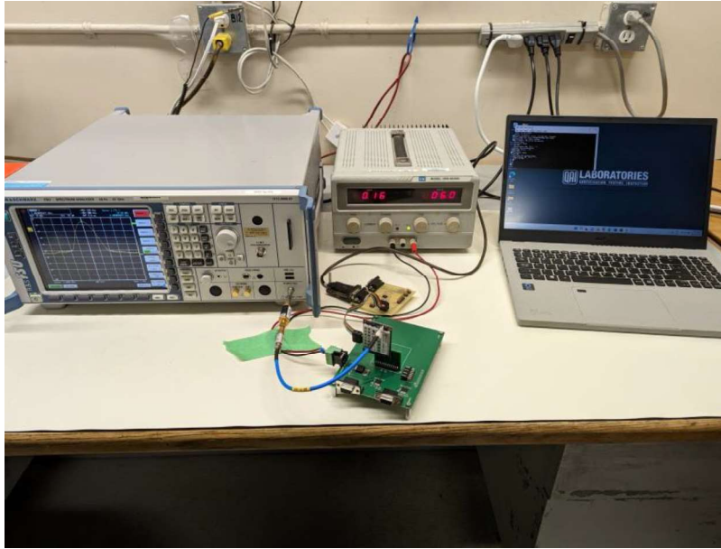
Figure 52: Peak Output Power Measurement Setup
