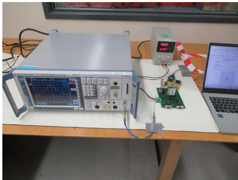
Figure 53: Other Conducted Radio Measurements Setup
