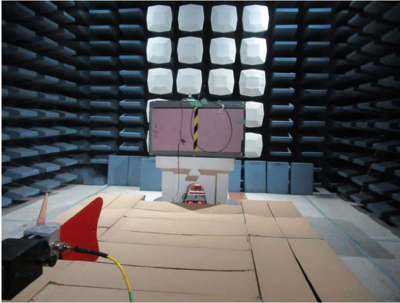
Figure 56: Radiated Emissions above 1 GHz, Measured at 3m Setup
