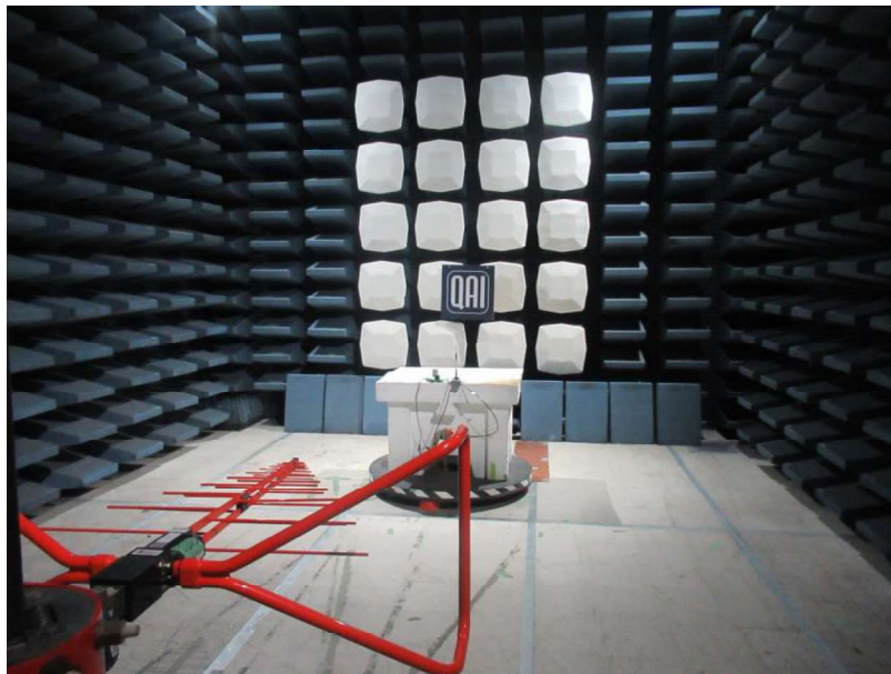
Figure 55: Radiated Emissions: 30 MHz - 1000 MHz, Measured at 3m Setup
