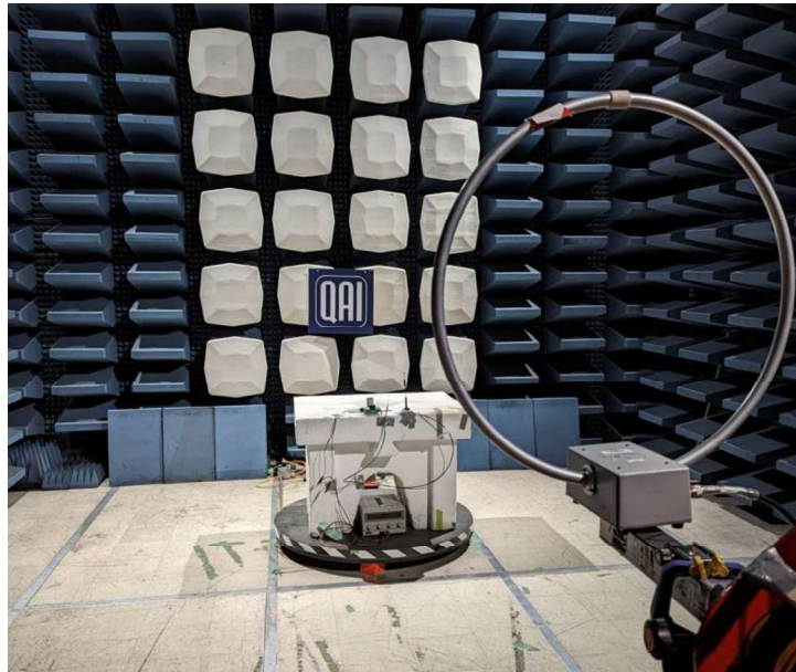
Figure 54: Radiated Emissions From 0.15 MHz - 30 MHz, Measured at 3m Setup
