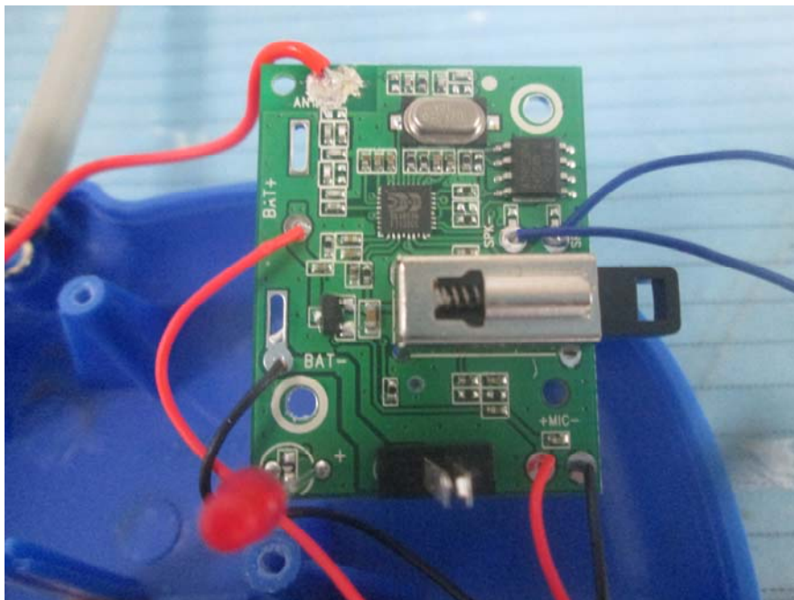
EUT –IC Main Chip 2 View
