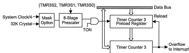
Timer Counter 3
