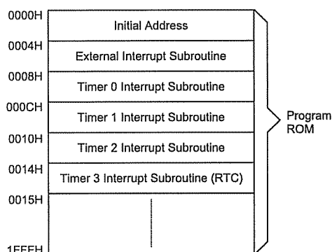
Program Memory
