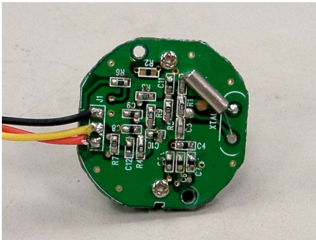
14. Front view of PCB 3
