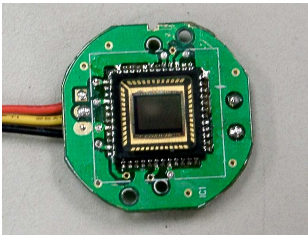
12. Front view of PCB 2
