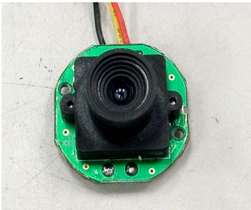
12. Front view of PCB 2
