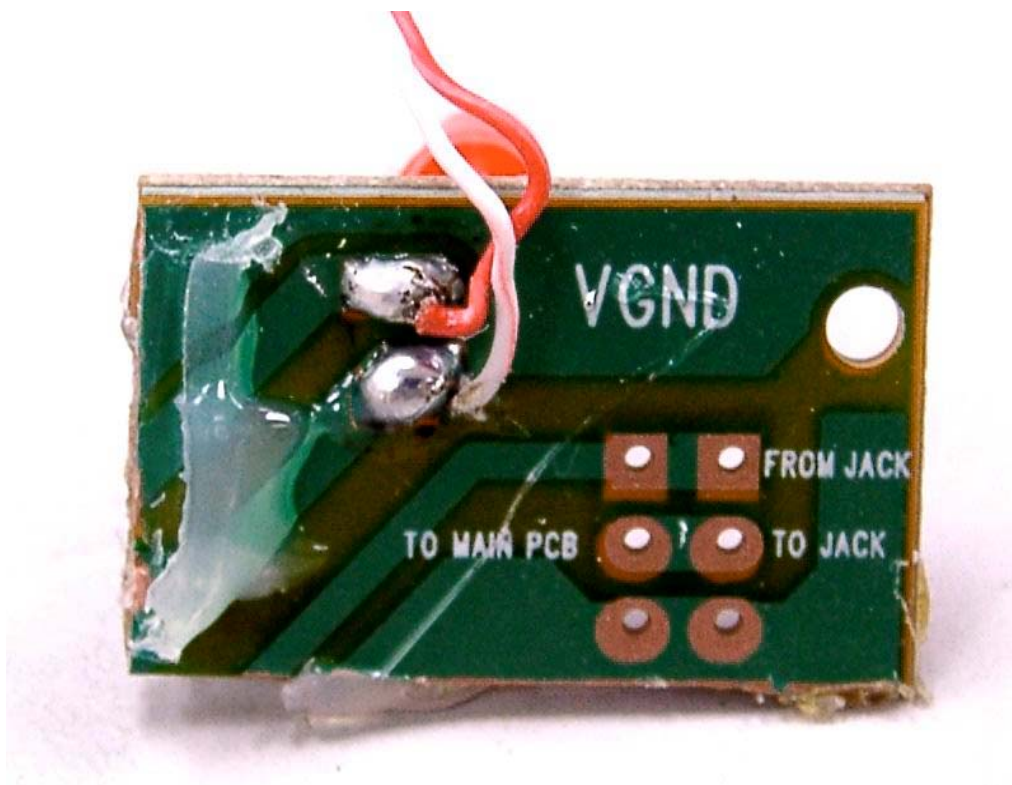
10. Rear view of PCB1
