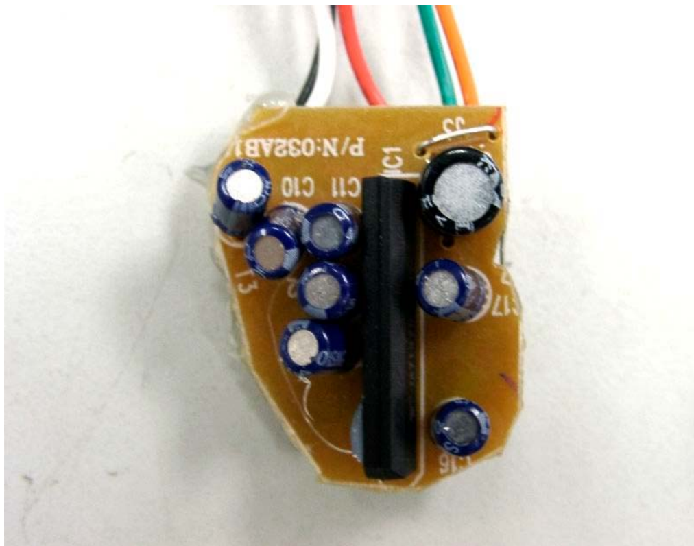
16. Front view of PCB 4
