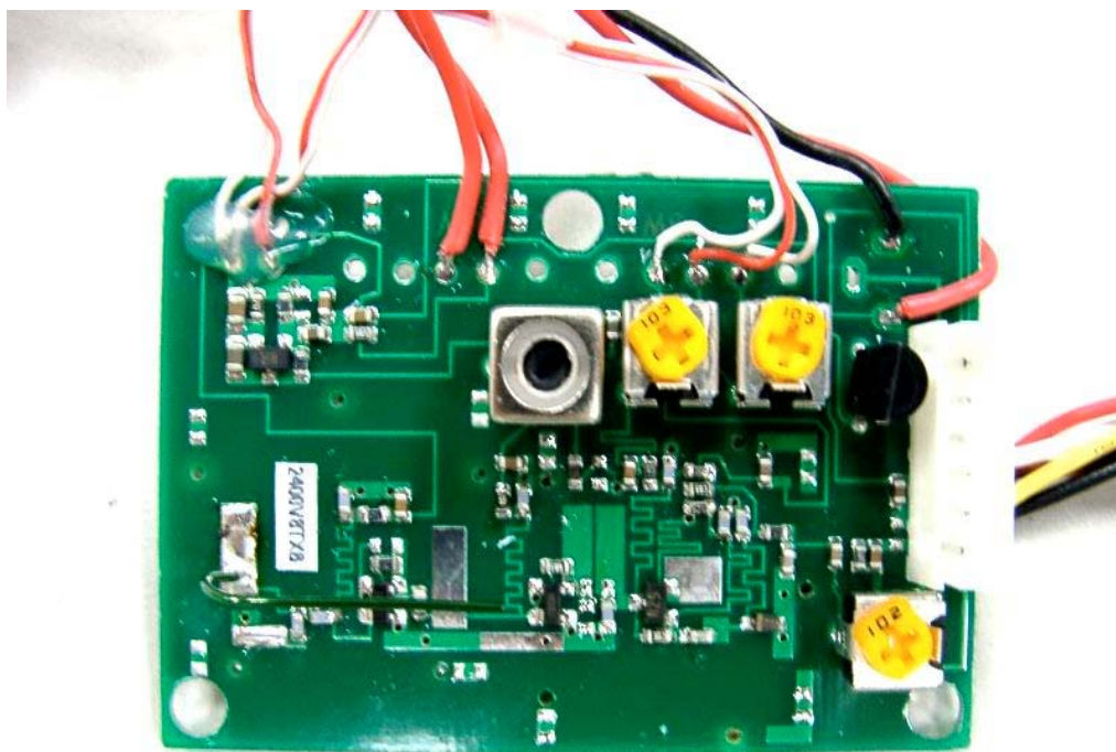
19. Front view of PCB 5
