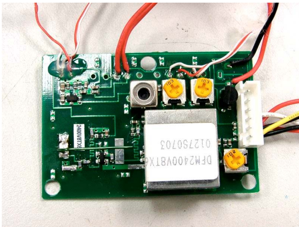
18. Front view of PCB 5
