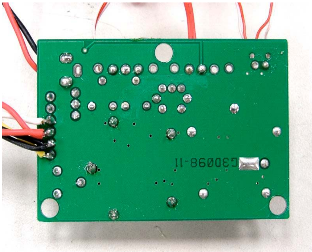
20. Rear view of PCB5
