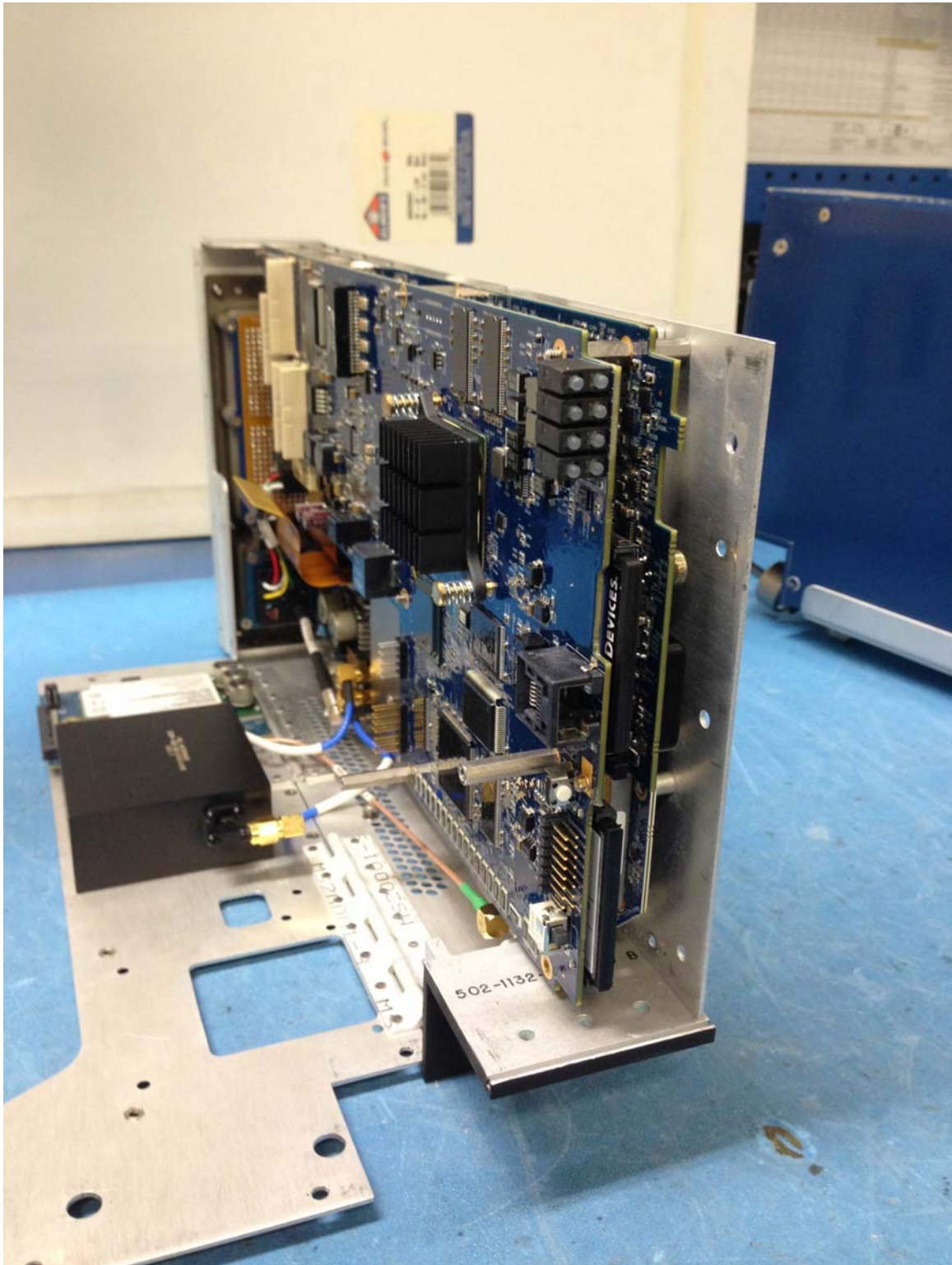
Figure 1: Front Panel Removed
