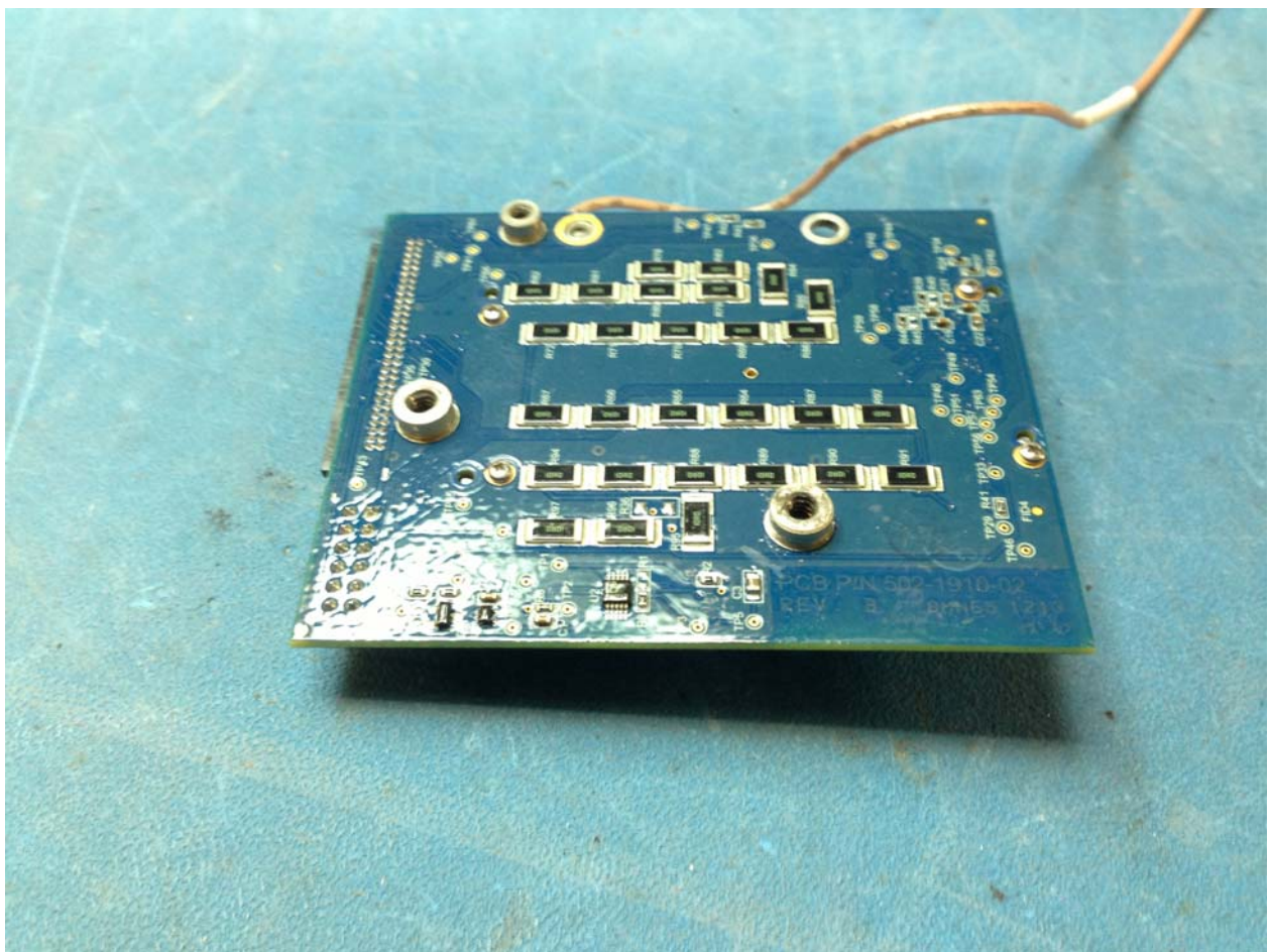
Figure 4: VMIM Board Bottom View
