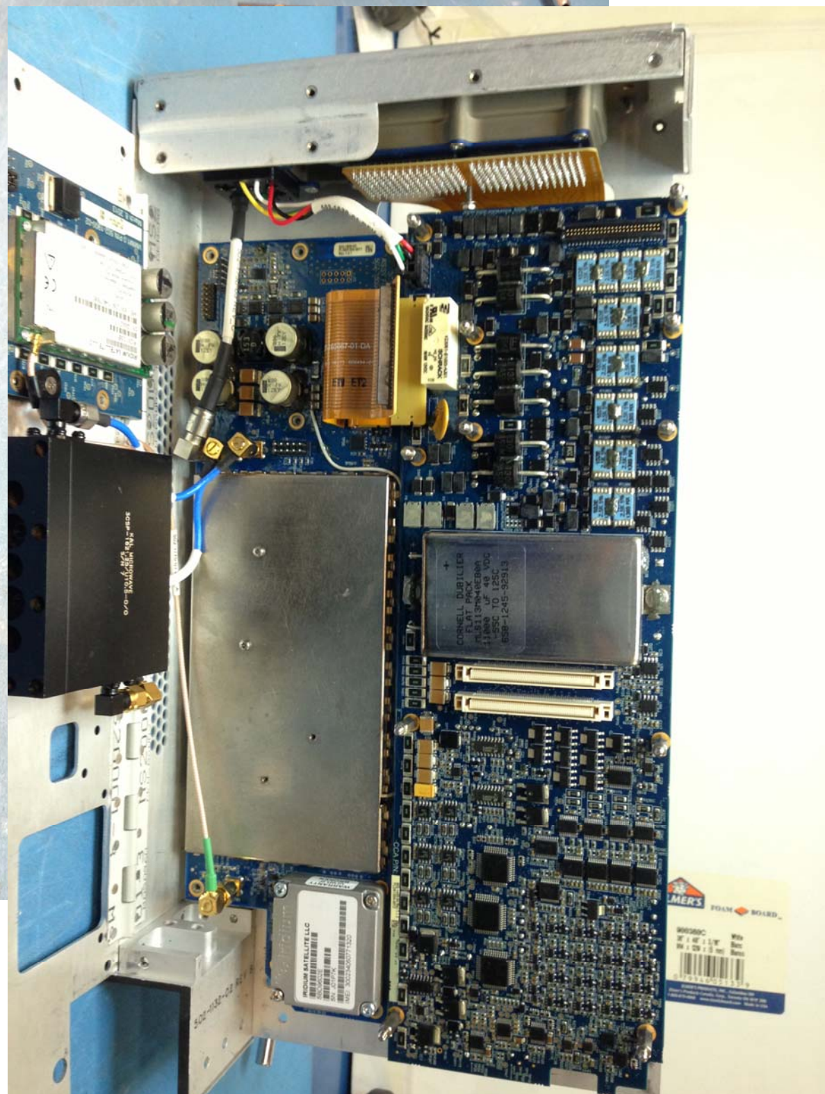
Figure 5: MCIM Board Removed
