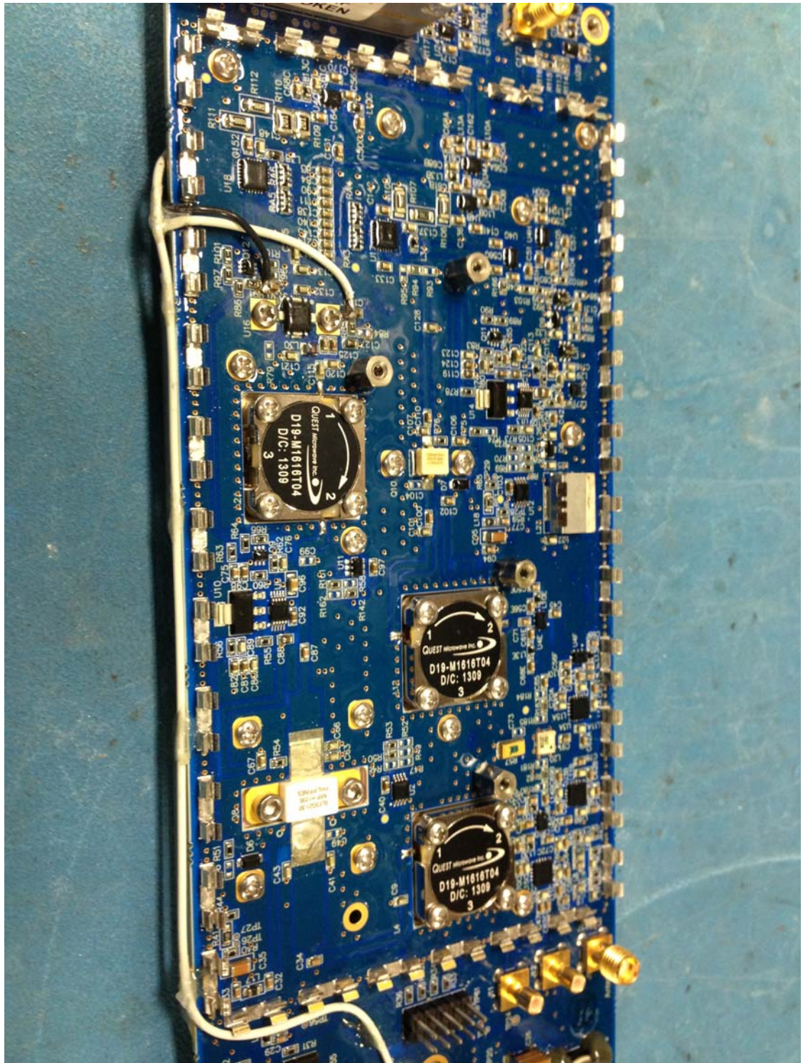
Figure 4: RFMM Board Top View (Circuitry Under the Metal Lid)
