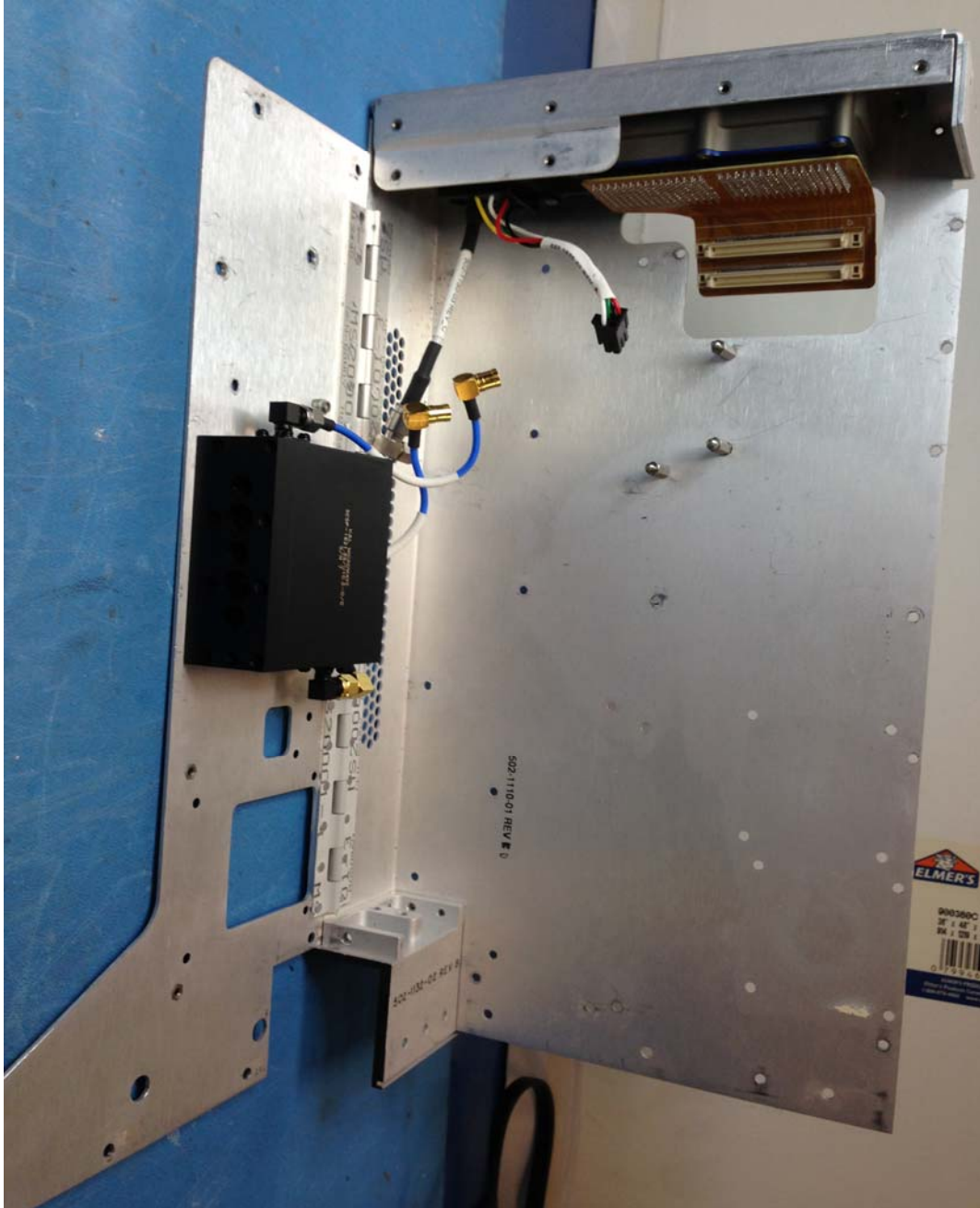
Figure 5: VMIM Board Removed
