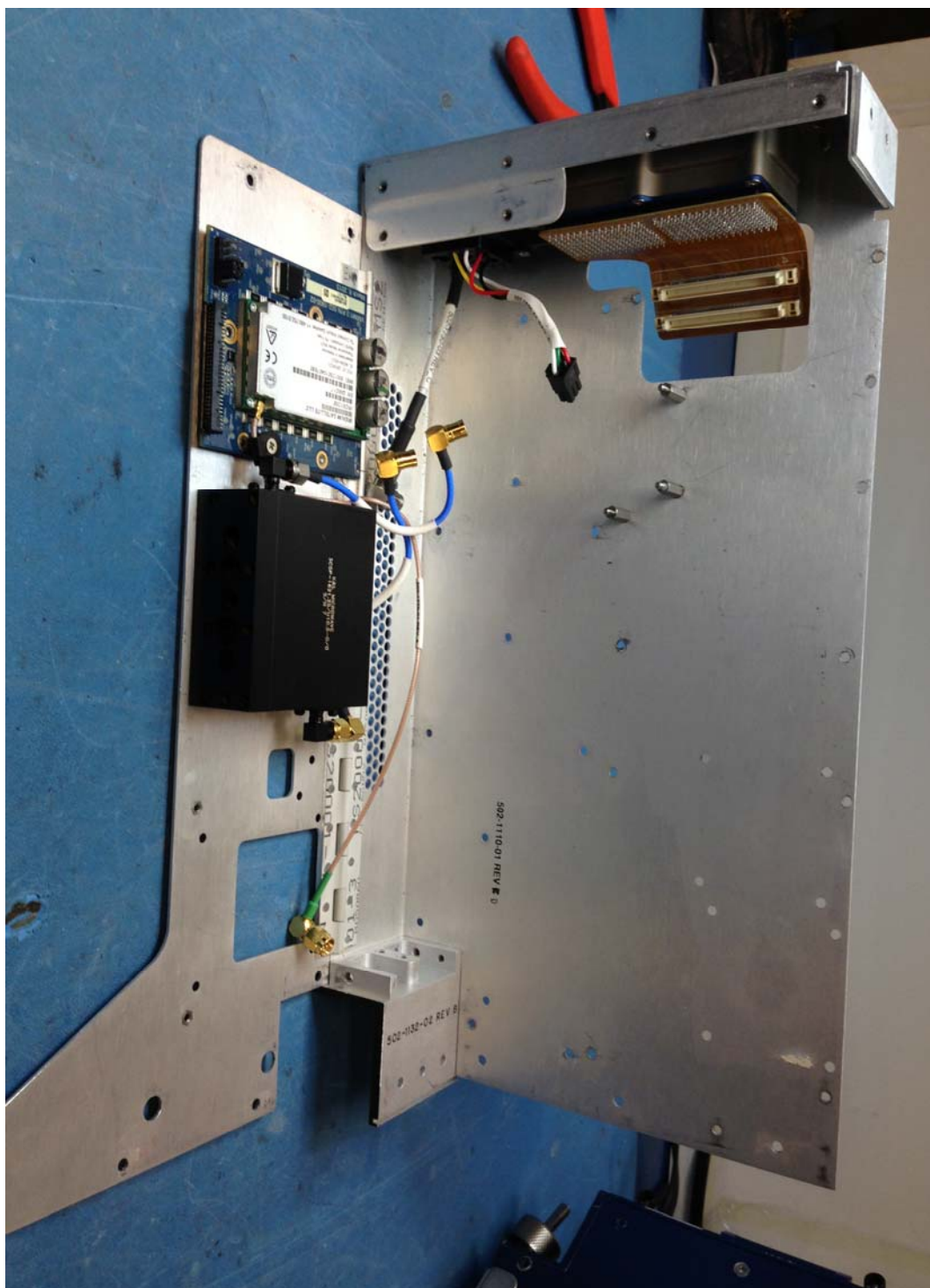
Figure 2: RFMM Board Removed
