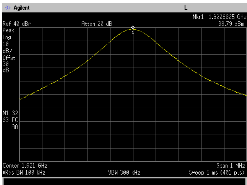
Output Power Plot 1620.9825 MHz
