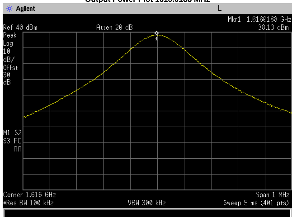
Output Power Plot 1616.0188 MHz
