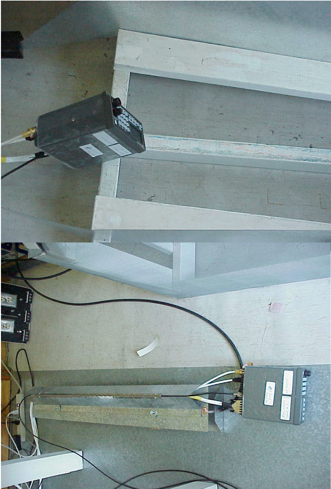
Radiated and Transient Immunity Test Setups
