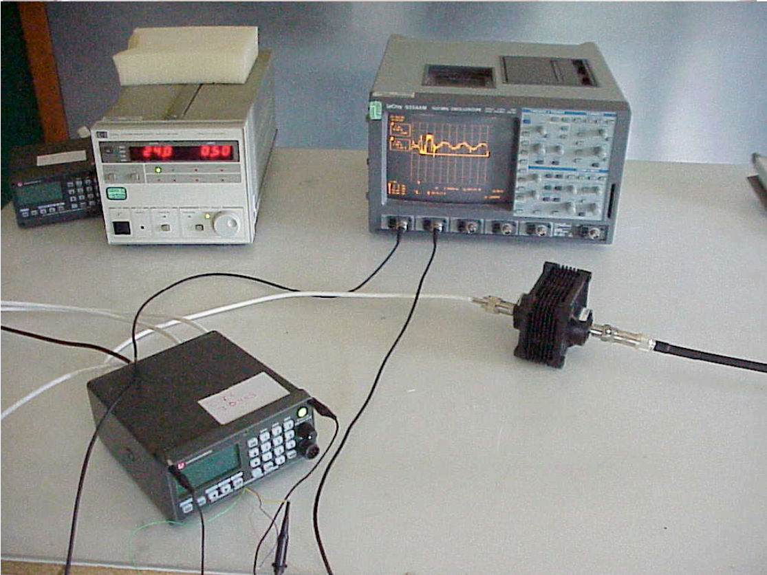
Sensitivity and T/R Switchtime Test Setups
