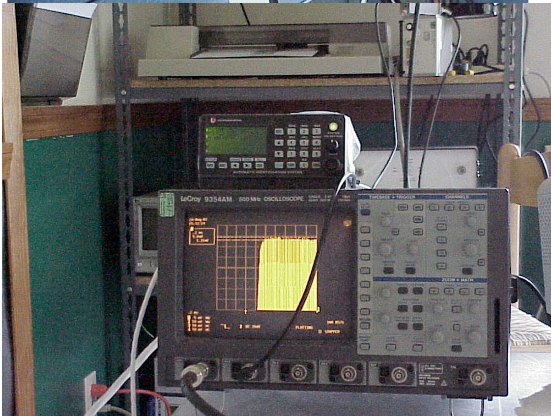
Intermodulation and Attack/Release Time Test Setup
