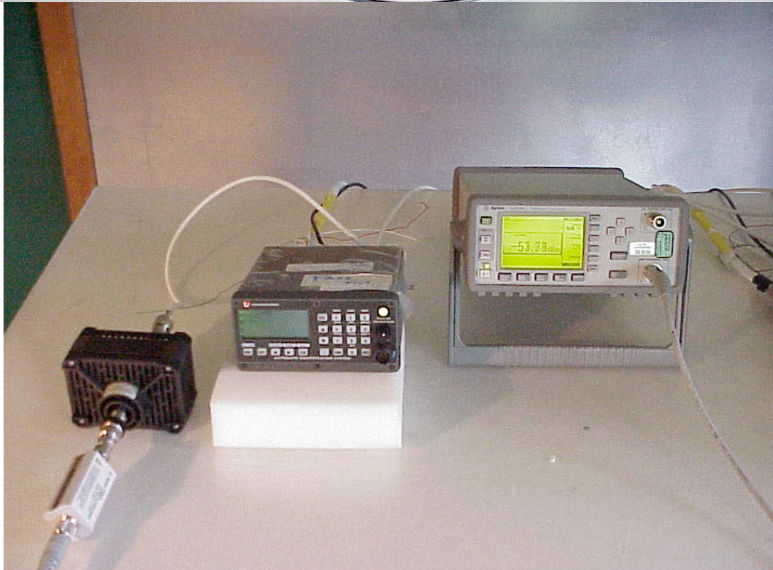
Frequency and Power Test Setups
