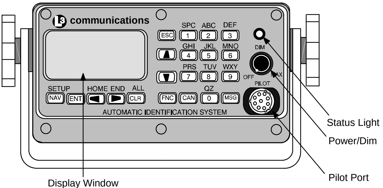
Figure 2-1. AIS Transponder
