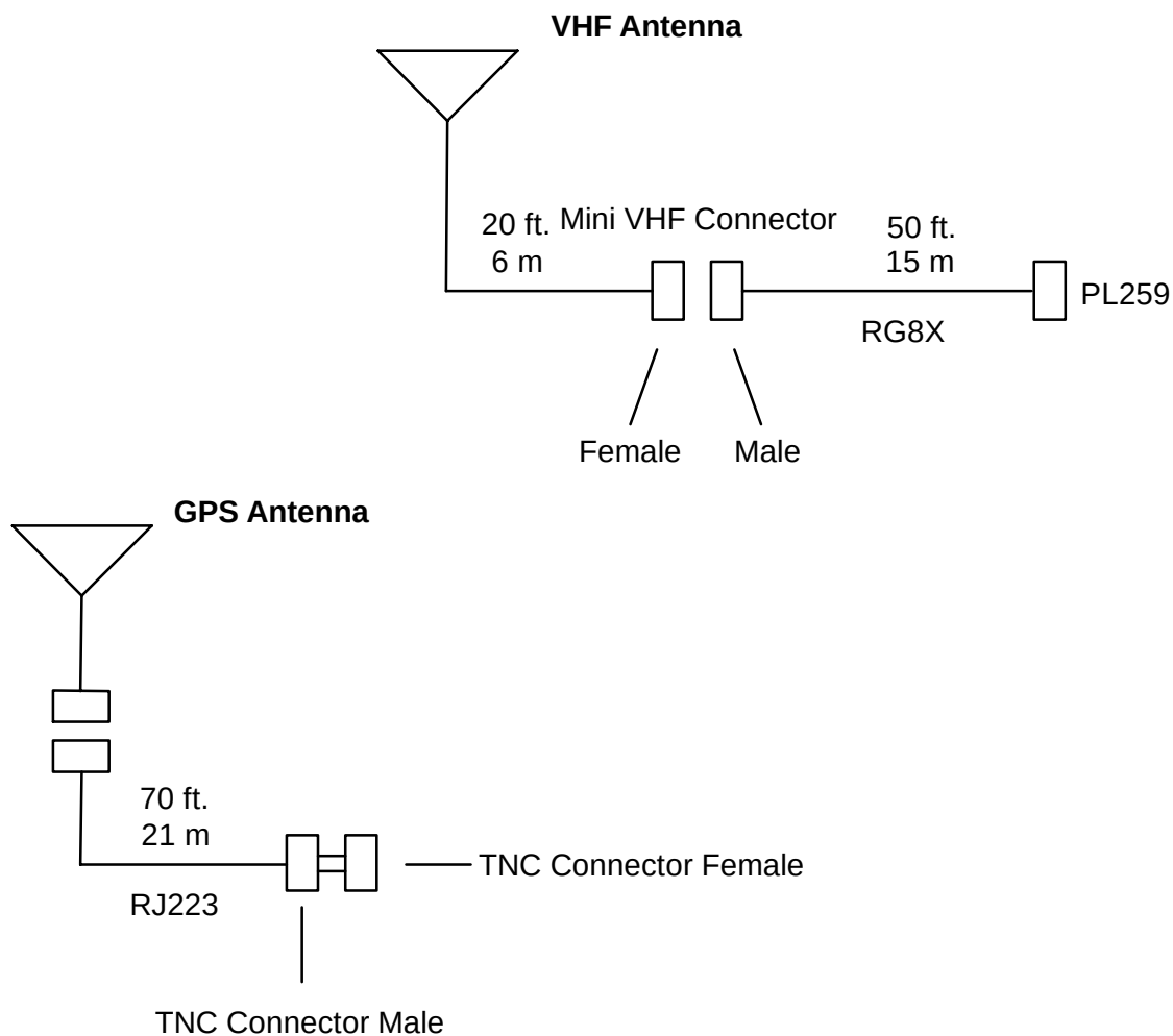
Figure 3-9. AIS Transponder Antenna Diagram
