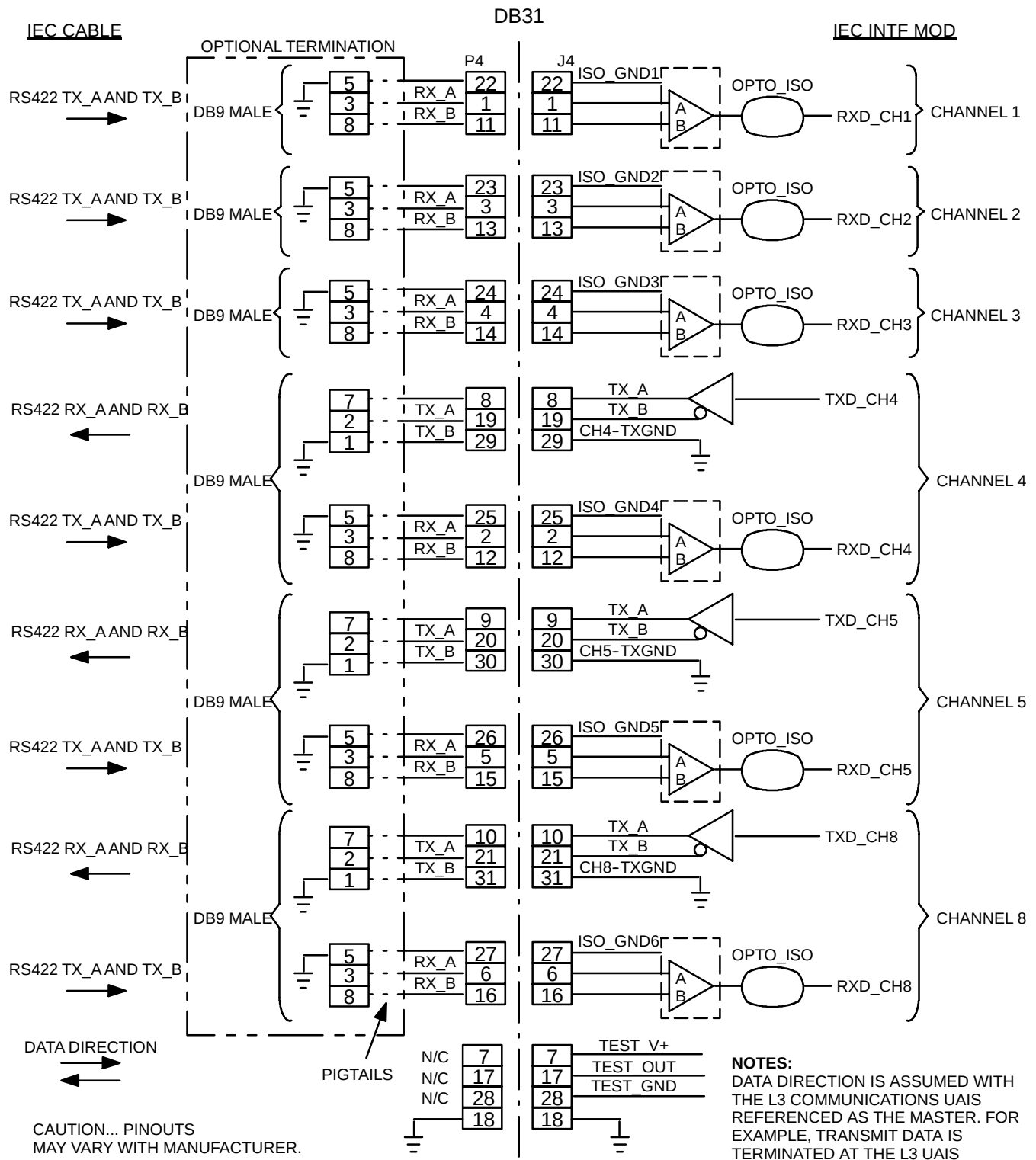
Figure 3-7. IEC Data Cable Interconnect Diagram
