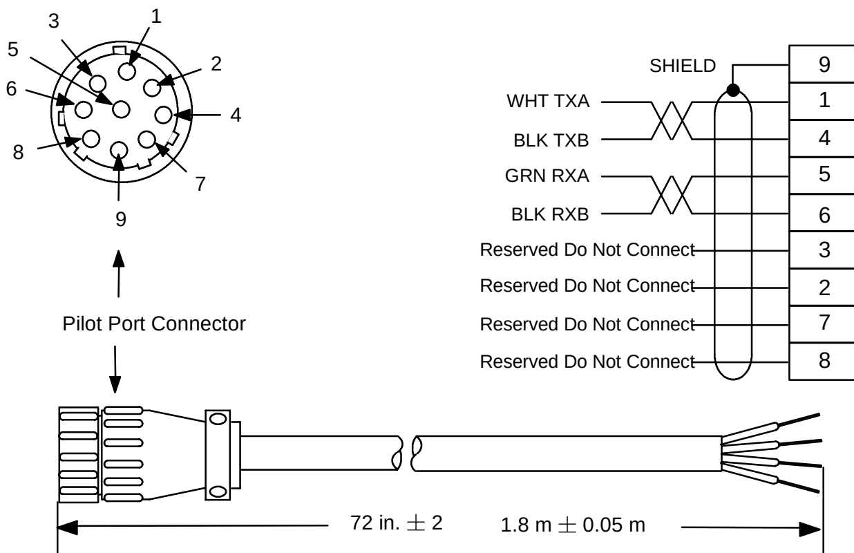
Figure 3-5. Pilot Port Cable
