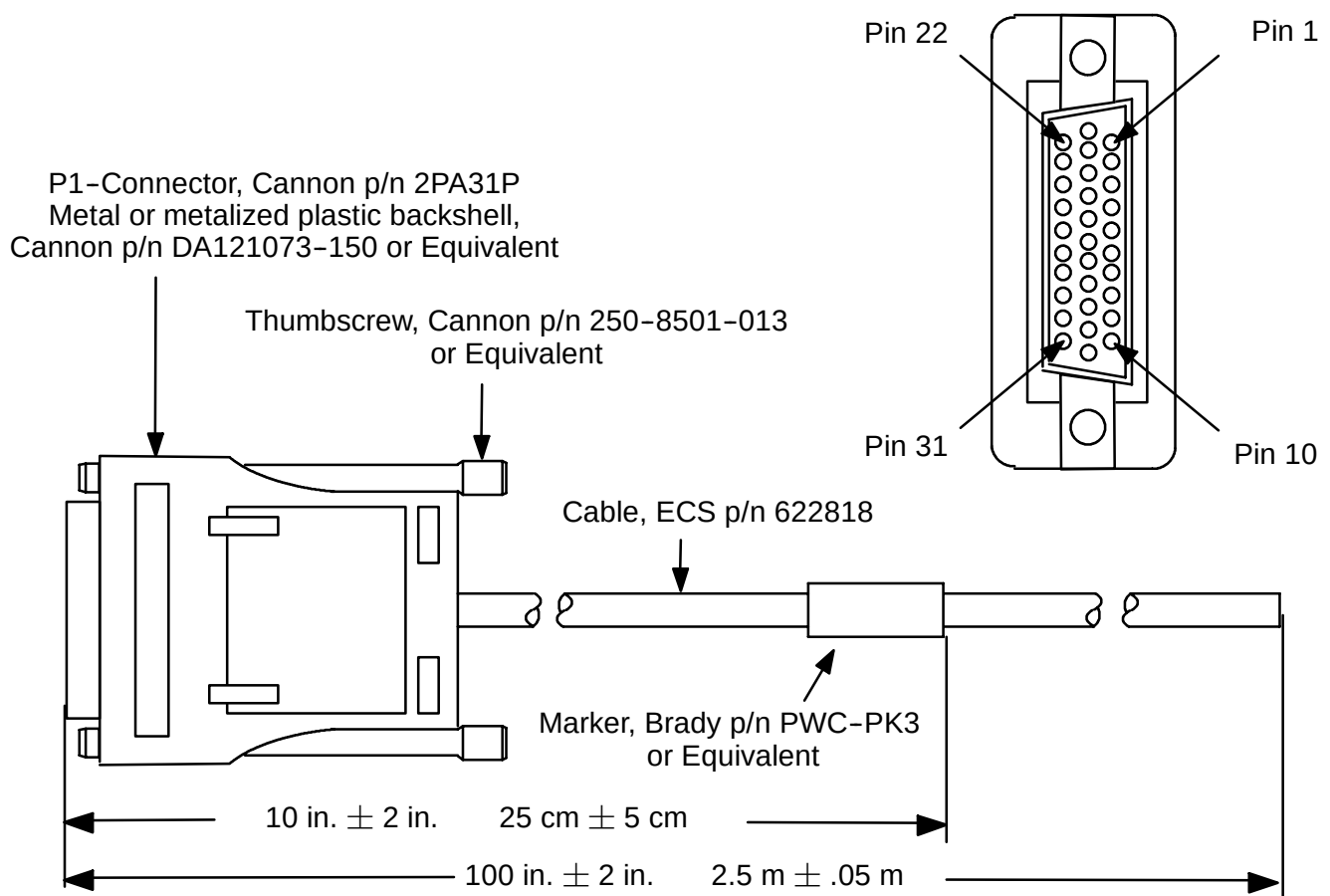
Figure 3-6. AIS Transponder IEC Data Cable
