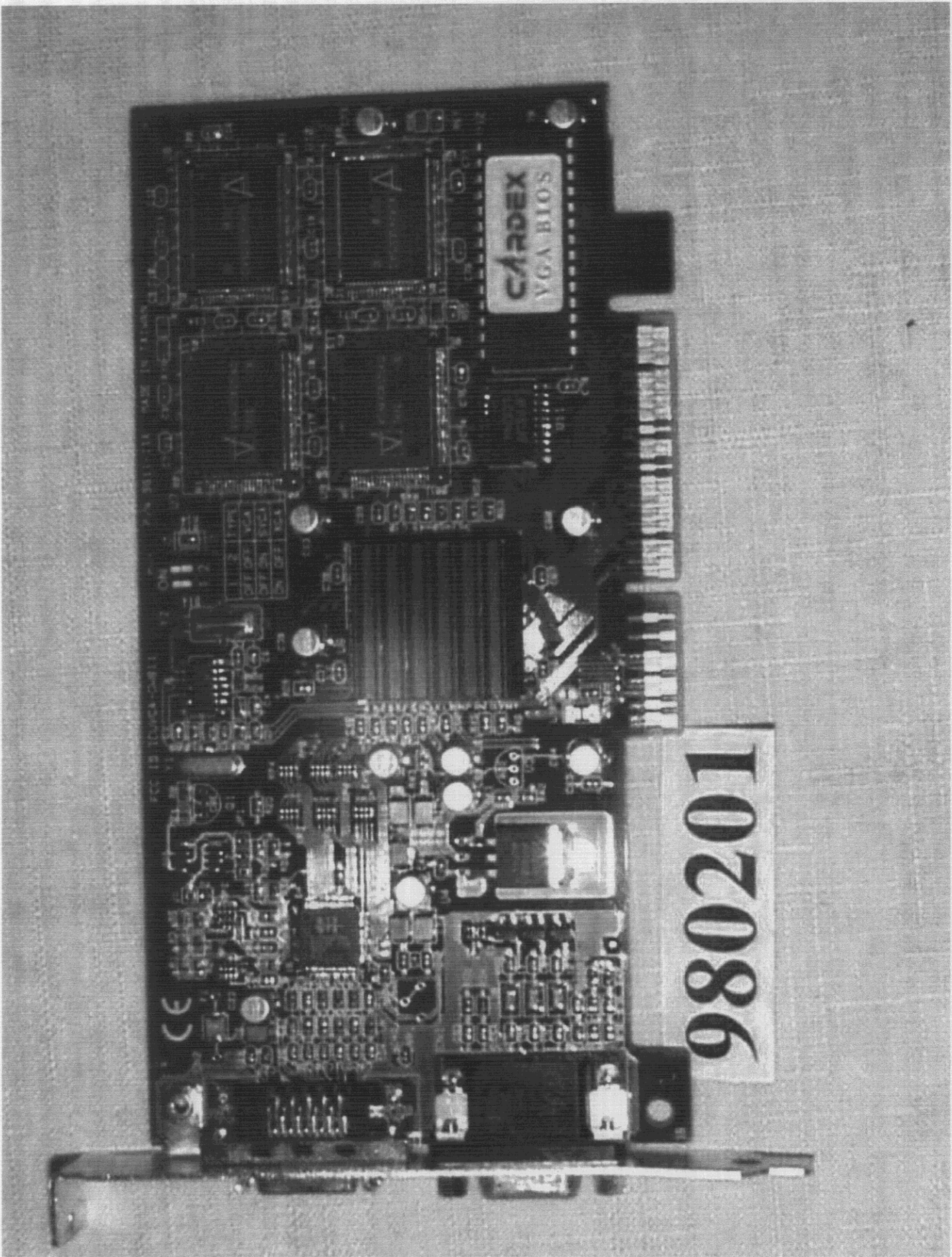
The Front View of EUT
