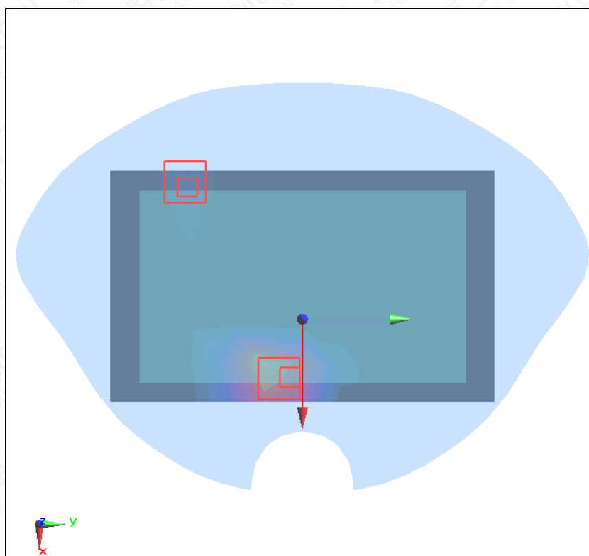
Figure A.1-22 LTE Band 5+Wi-Fi5G Back 0mm
