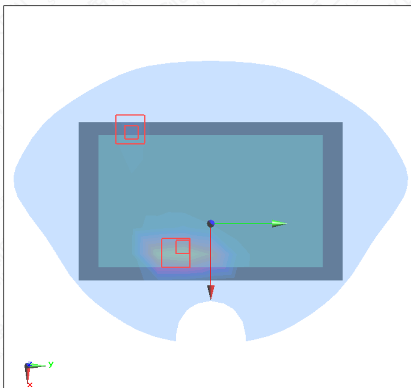
Figure A.1-26 LTE Band 13+Wi-Fi5G Back 0mm
