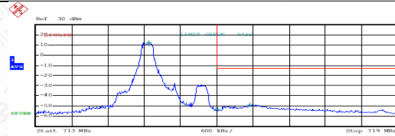
FDD12HighRange_1.4MHz_QPSK_OneRB _low
