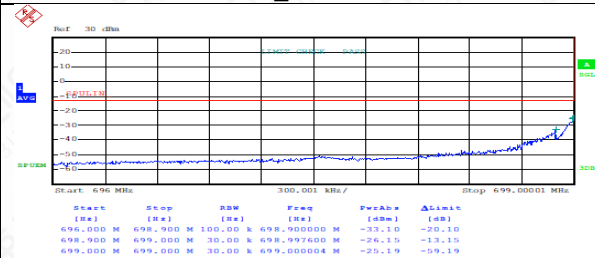
FDD12LowRange_1.4MHz_QPSK_OneRB _low
