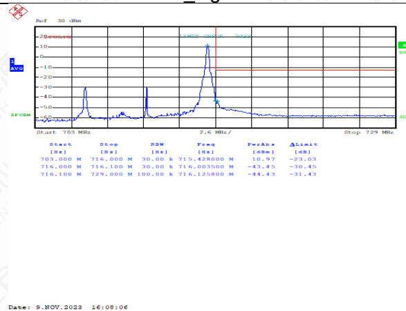
FDD12HighRange_10MHz_QPSK_OneRB high
