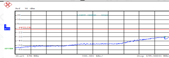
FDD12LowRange_1.4MHz_QPSK_FullRB _Low
