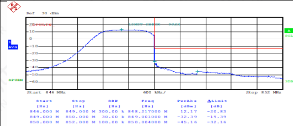
FDD05HighRange_1.4MHz_QPSK_FullRB _High
