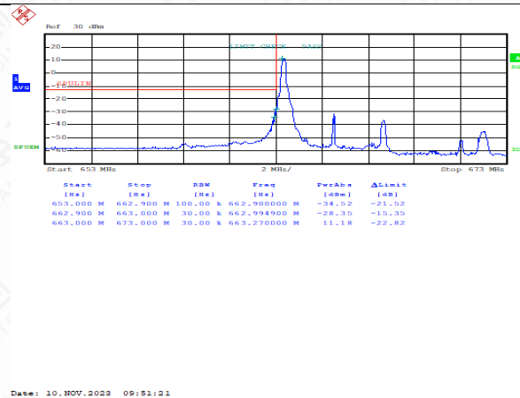
FDD71HighRange_20MHz_QPSK_OneRB high
