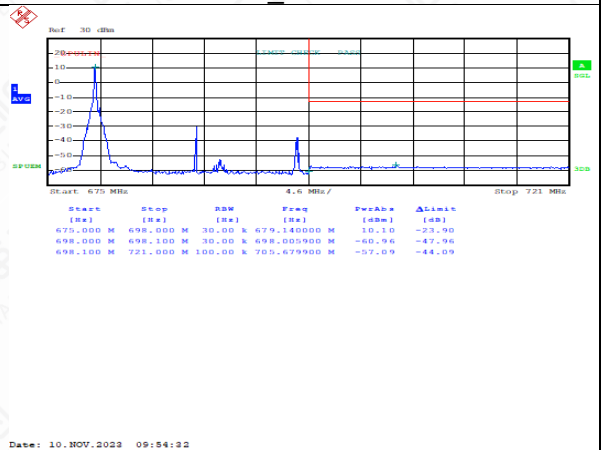
FDD71HighRange_20MHz_QPSK_OneRB low
