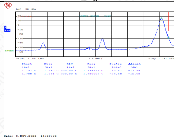
FDD66HighRange_20MHz_QPSK_OneRB high
