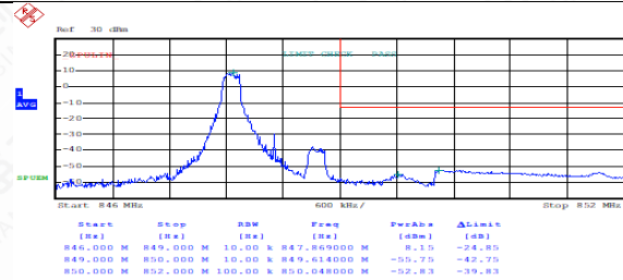
FDD05HighRange_1.4MHz_QPSK_OneRB _low
