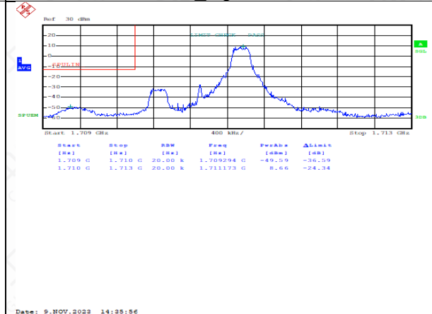
FDD66LowRange_1.4MHz_QPSK_FullRB Low
