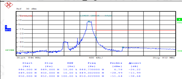
FDD05HighRange_1.4MHz_QPSK_OneRB _high
