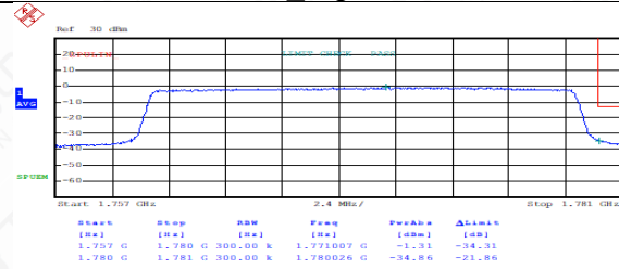
FDD66HighRange_20MHz_QPSK_FullRB_High
