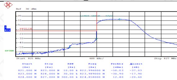
FDD05LowRange_1.4MHz_QPSK_FullRB _Low
