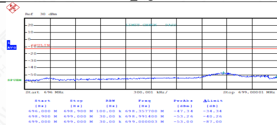
FDD12LowRange_1.4MHz_QPSK_OneRB _high
