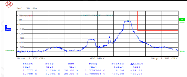
FDD66HighRange_1.4MHz_QPSK_OneRB_high
