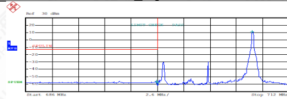
FDD12LowRange_10MHz_QPSK_OneRB _high
