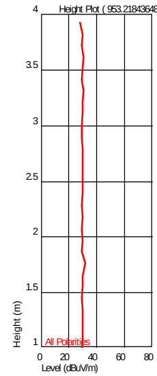
Height Plot ( 953.218436487 MHz )
