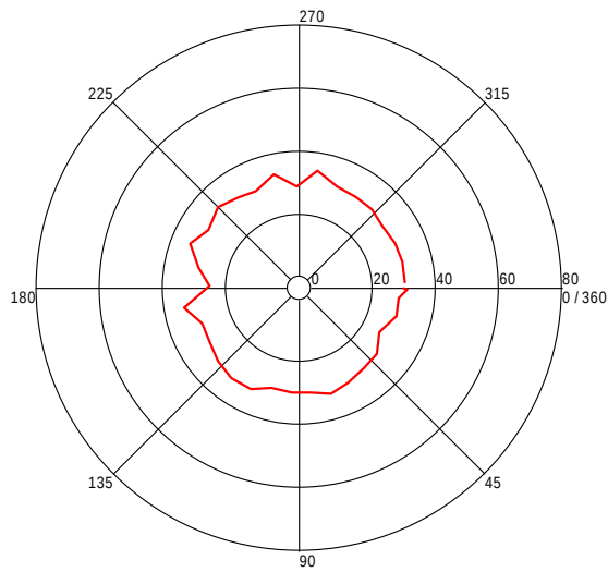
Turntable Plot ( 833.171141982 MHz )
