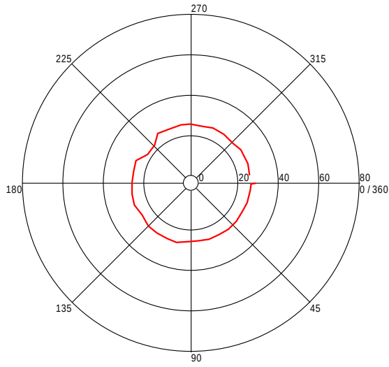
Turntable Plot ( 31.400000112 MHz )
