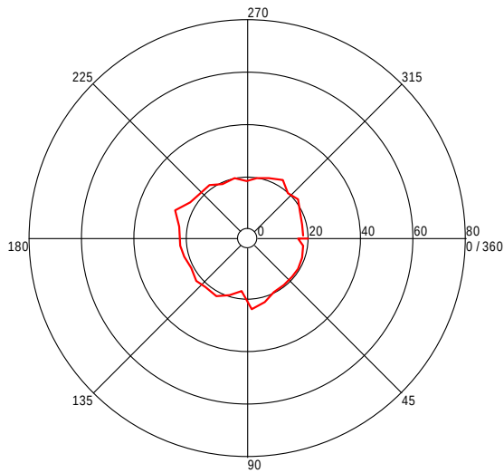
Turntable Plot ( 42.934268996 MHz )
