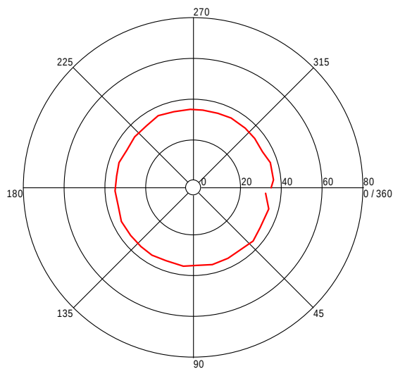
Turntable Plot ( 1.296158984 GHz )
