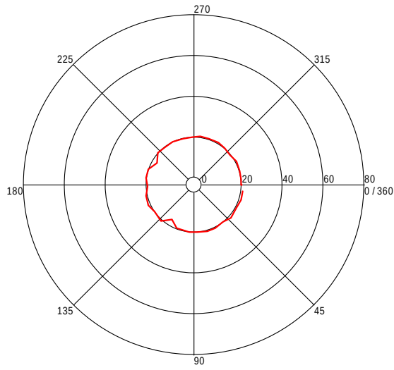
Turntable Plot ( 129.564729906 MHz )
