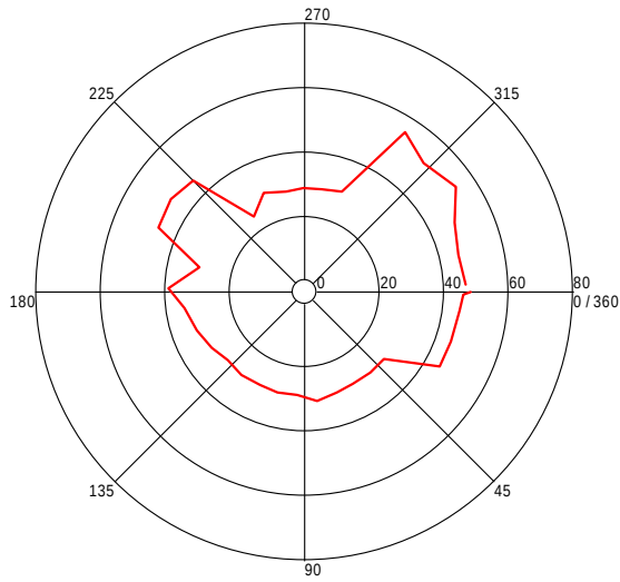
Turntable Plot ( 832.851101846 MHz )
