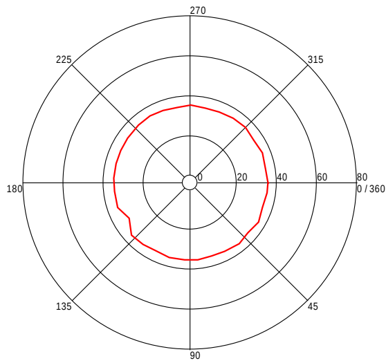
Turntable Plot ( 1.227768871 GHz )
