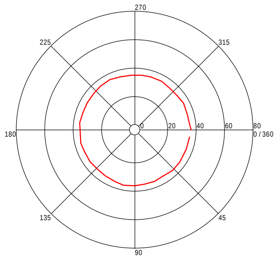
Turntable Plot ( 1.268463594 GHz )
