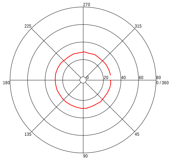
Turntable Plot ( 706.143487082 MHz )
