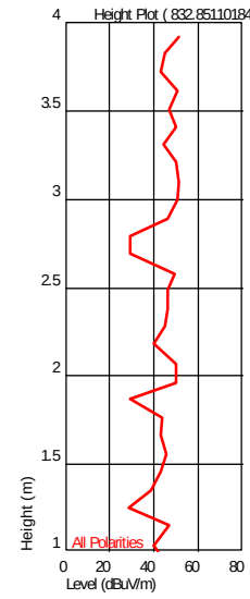
Height Plot ( 832.851101846 MHz )
