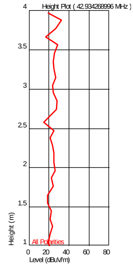
Height Plot ( 42.934268996 MHz )
