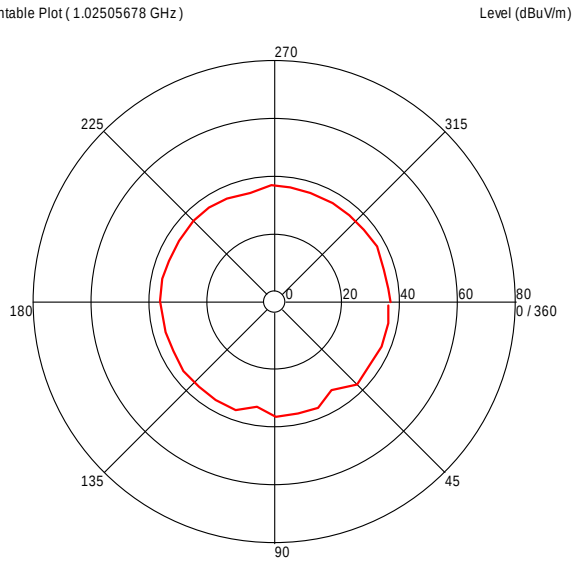
Turntable Plot ( 1.02505678 GHz )
