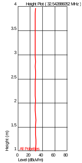
Height Plot ( 32.542886052 MHz )
