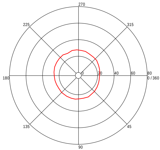
Turntable Plot ( 210.63747488 MHz )
