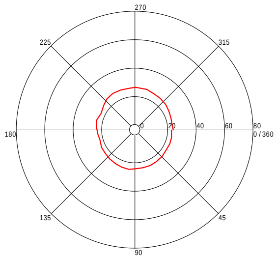
Turntable Plot ( 361.515631587 MHz )
