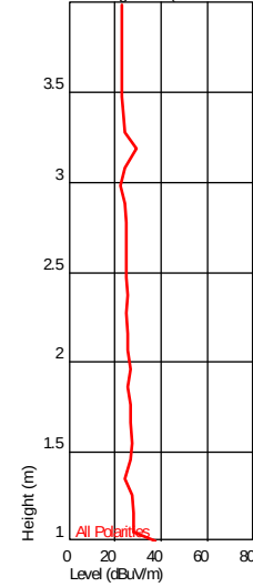
Height Plot ( 210.63747488 MHz )
