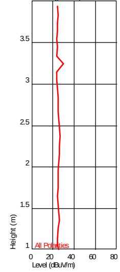
Height Plot ( 63.33005992 MHz )
