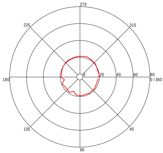
Turntable Plot ( 174.470140002 MHz )
