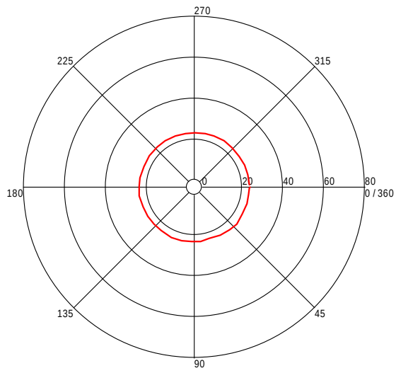
Turntable Plot ( 63.33005992 MHz )
