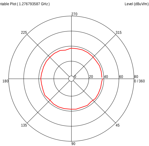
Turntable Plot ( 1.276793587 GHz )
