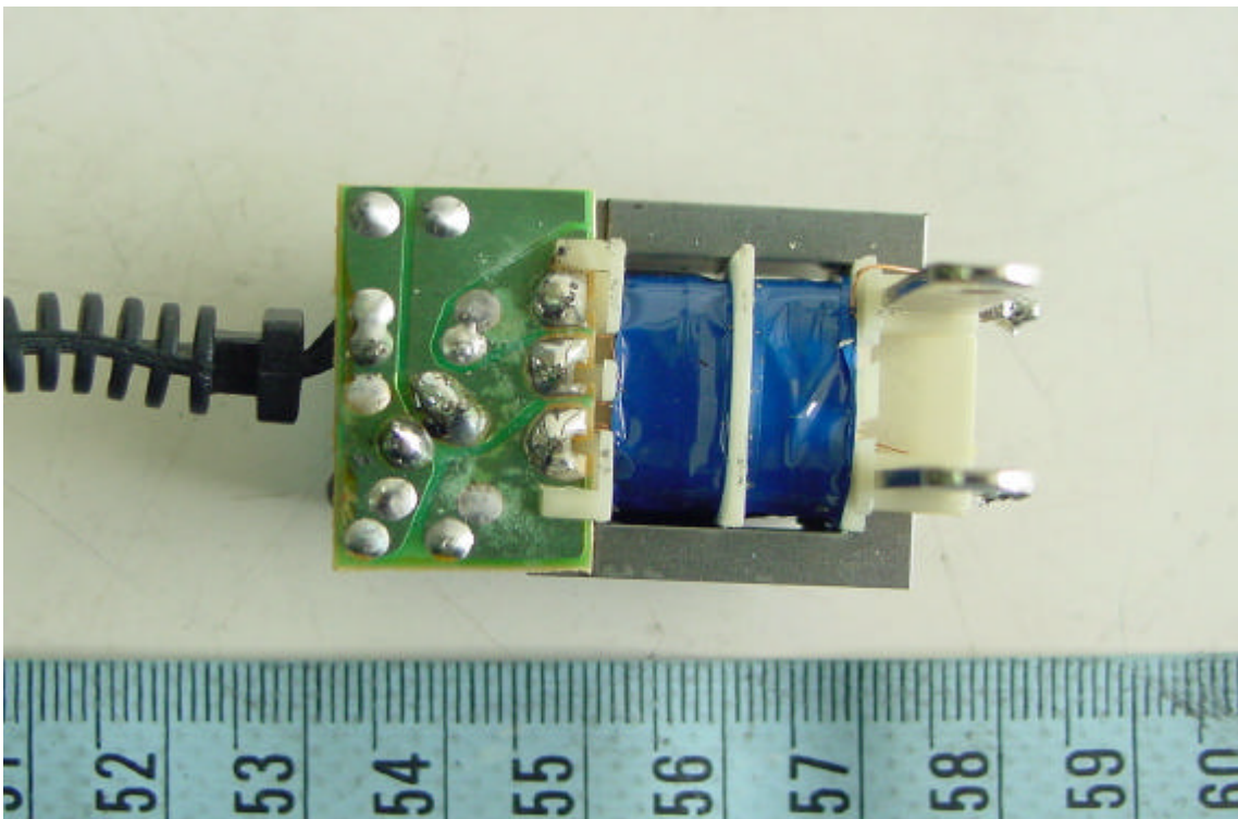
Solder View of Adapter 's Main PCB
