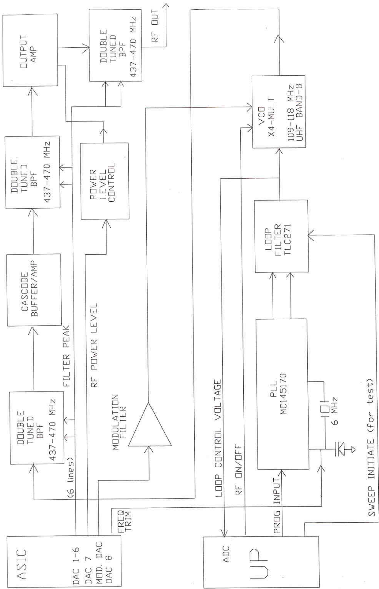
TRANSMITTER (RF section)
