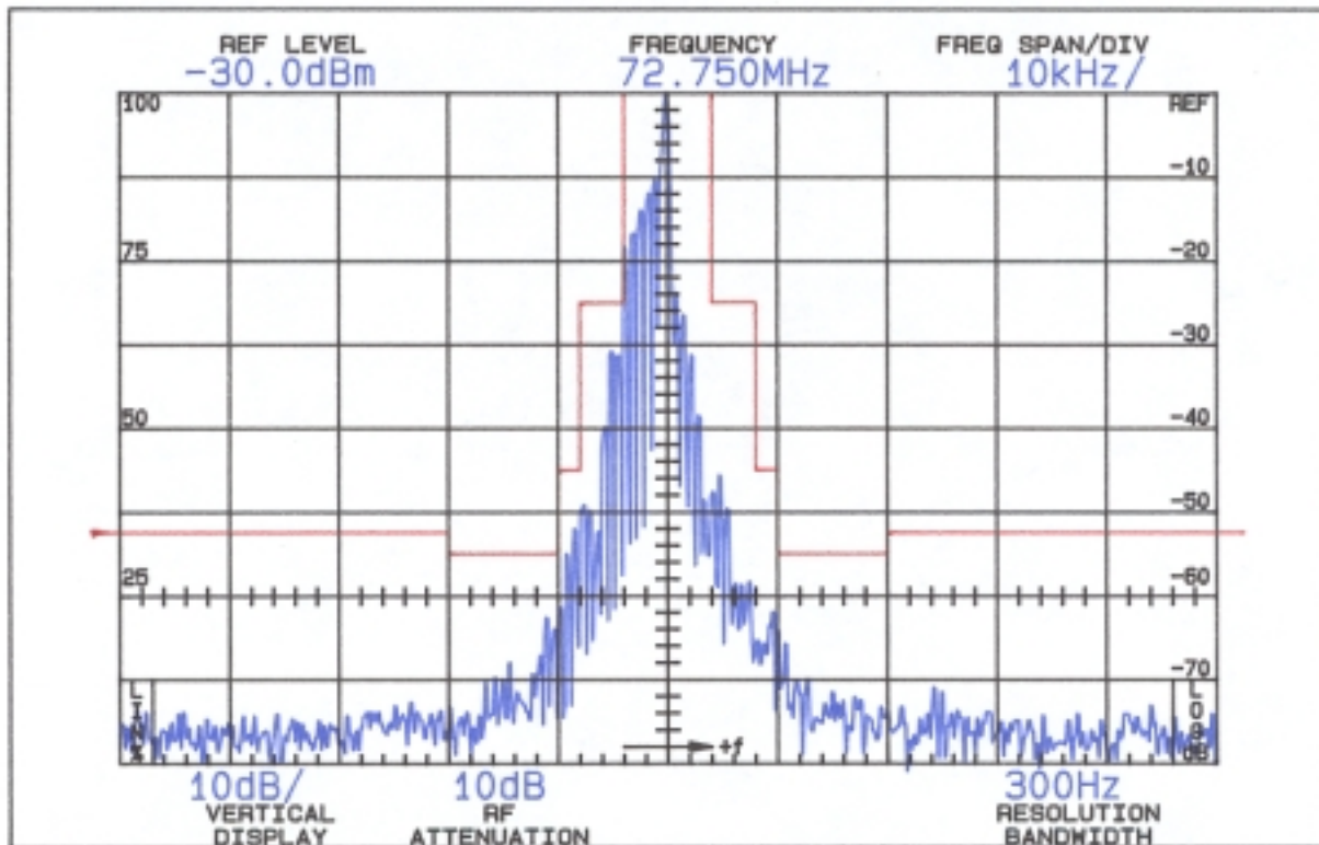
FIGURE 1 OCCUPIED BANDWIDTH
