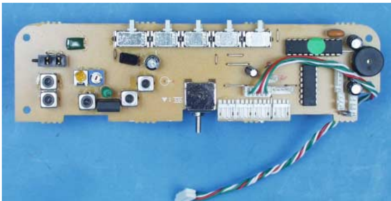
Circuit Board – Component Side
