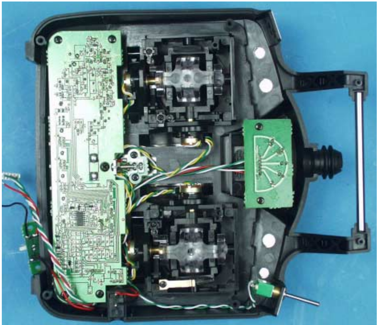
Circuit Board
