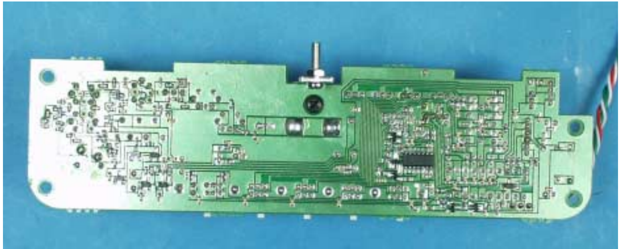
Circuit Board – Track Side
