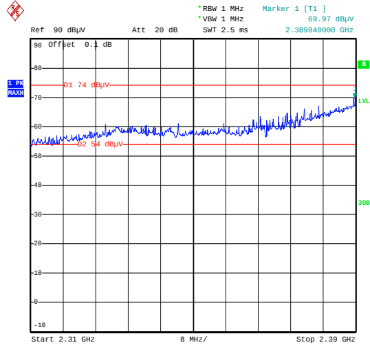
Lowest Channel(2 409.2 MHz): PEAK
