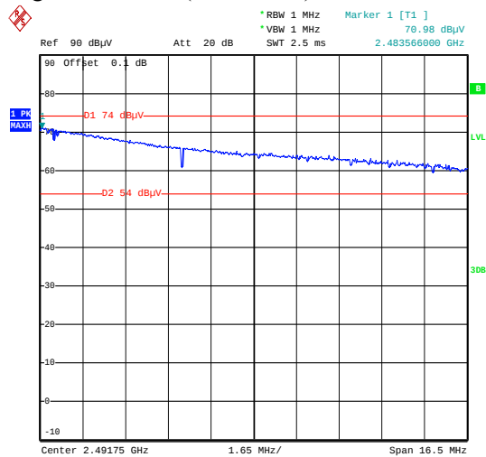
Highest Channel(2 474.0 MHz): PEAK
