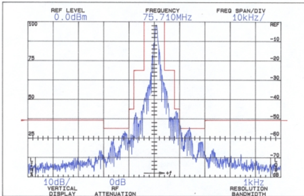
FIGURE 1 OCCUPIED BANDWIDTH
