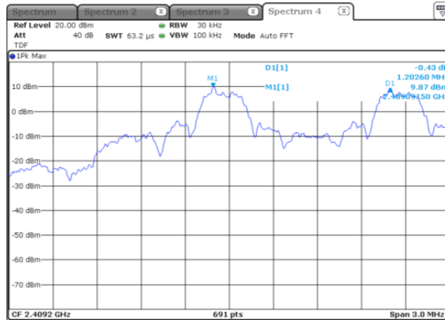
Figure 2. Plot of the Carrier Frequency Separation (Conducted)
