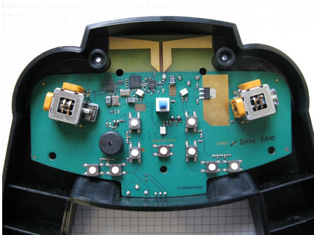
Smart SX PCB TOP
