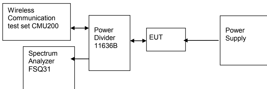
Figure 4. Test Set-up
