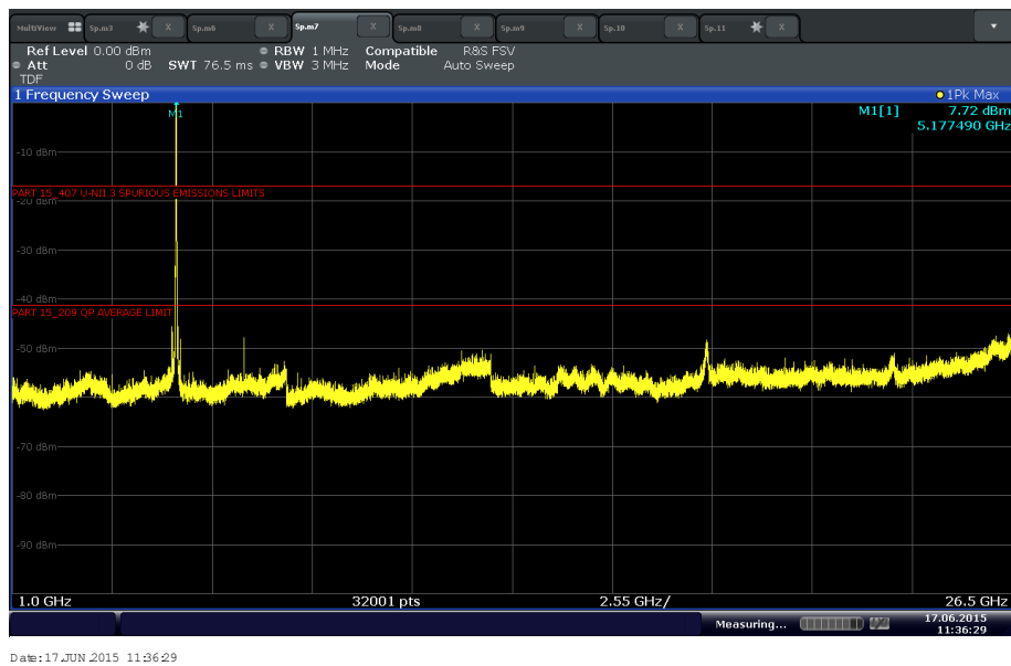
U-NII 1 802.11 n Low Channel above 1GHz (20 MHz BW)
