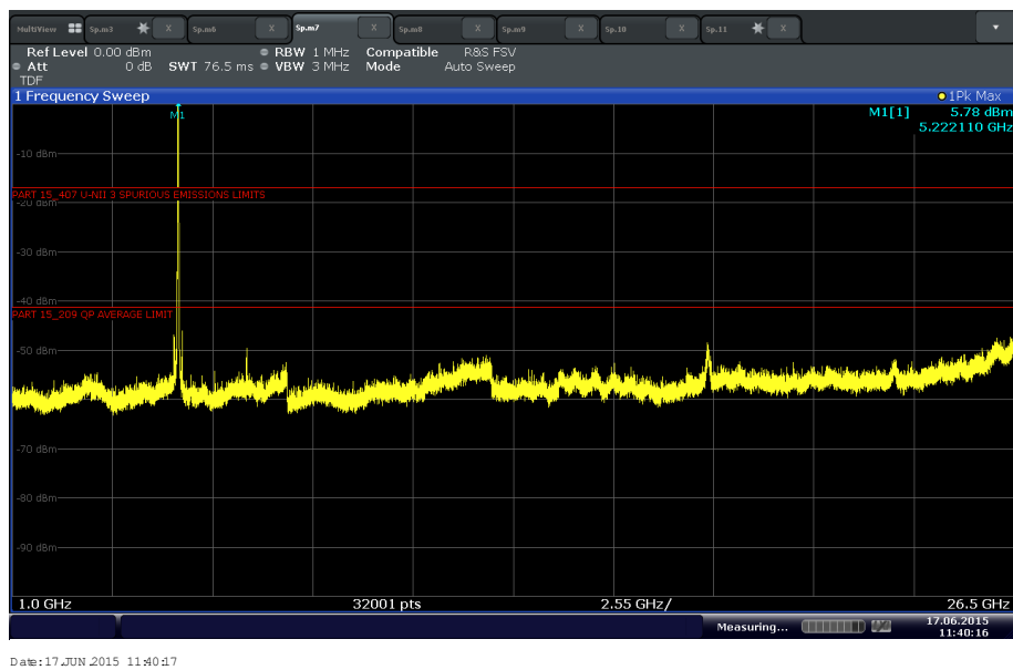
U-NII 1 802.11 n Mid Channel above 1GHz (20 MHz BW)
