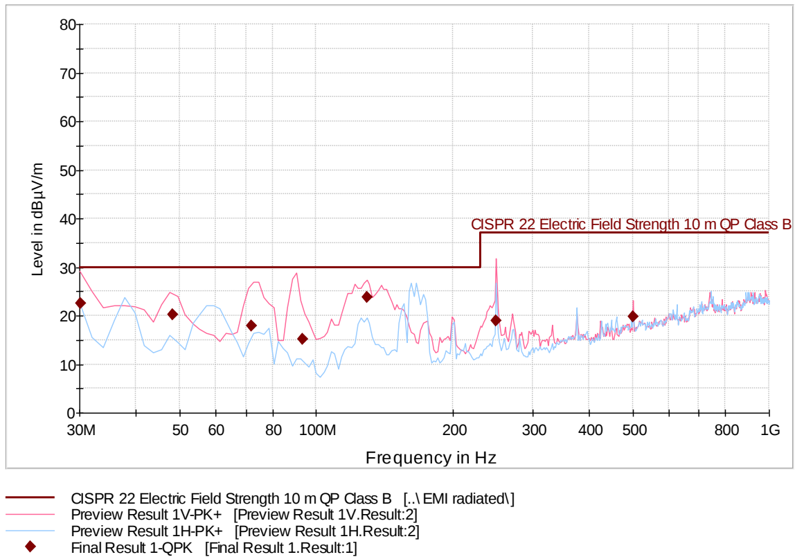
Continuous Rotation TUV 10m Radiated 30 to 1000MHz
