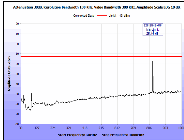
Plot 37. Radiated Spurious Emissions, GPRS, 850 MHz Band, Low Channel, 30 MHz – 1 GHz
