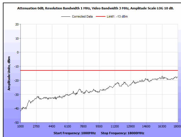
Plot 66. Radiated Spurious Emissions, WCDMA, 850 MHz Band, High Channel, 1 GHz – 18 GHz
