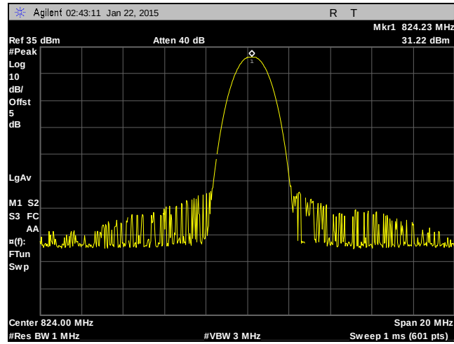
Plot 1. RF Power, GPRS, 850 MHz Band, Low Channel
