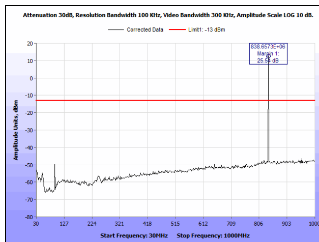
Plot 39. Radiated Spurious Emissions, GPRS, 850 MHz Band, Mid Channel, 30 MHz – 1 GHz
