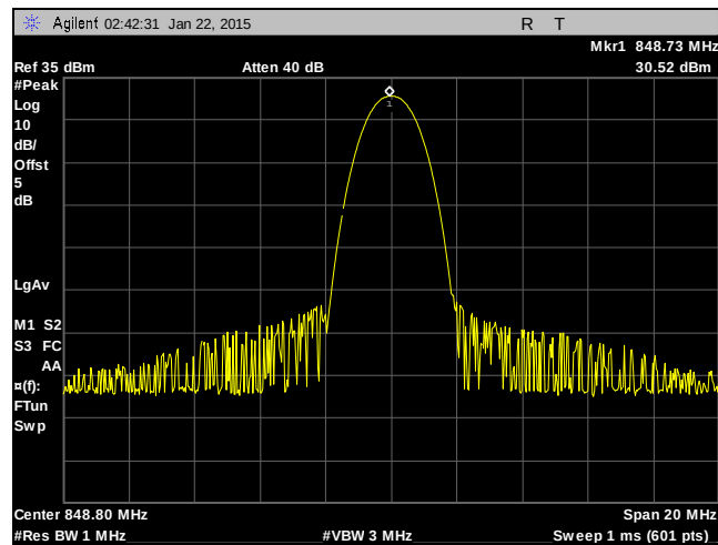
Plot 3. RF Power, GPRS, 850 MHz Band, High Channel
