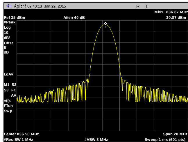
Plot 2. RF Power, GPRS, 850 MHz Band, Mid Channel
