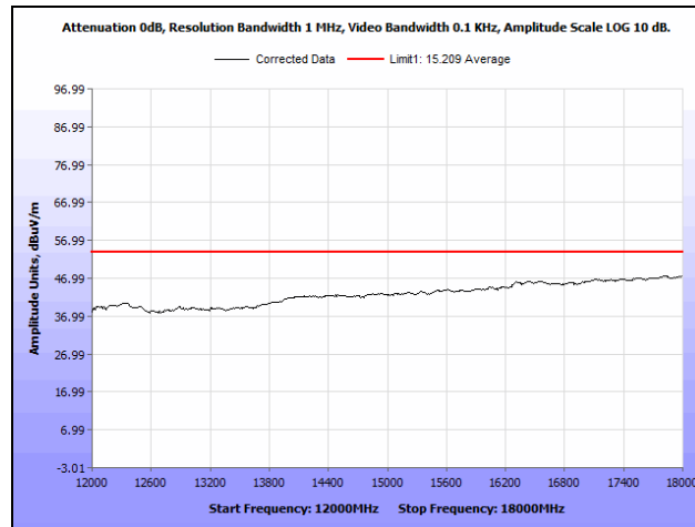
Plot 35. Radiated Spurious Emissions, Mid Channel, 12 GHz – 18 GHz, Average
