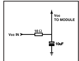
figure 10: Supply Filter
