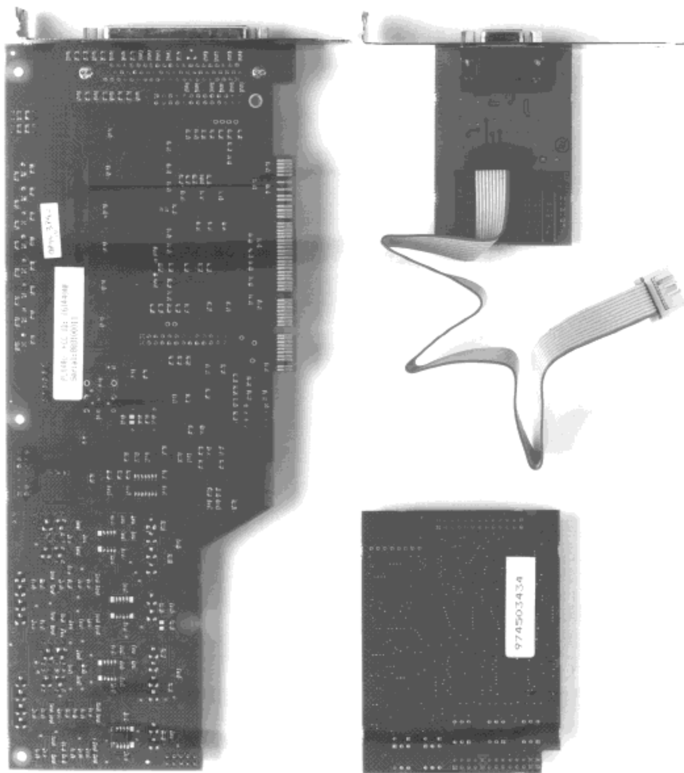
Figure 8.1 PCX440np Board, Foil Side
