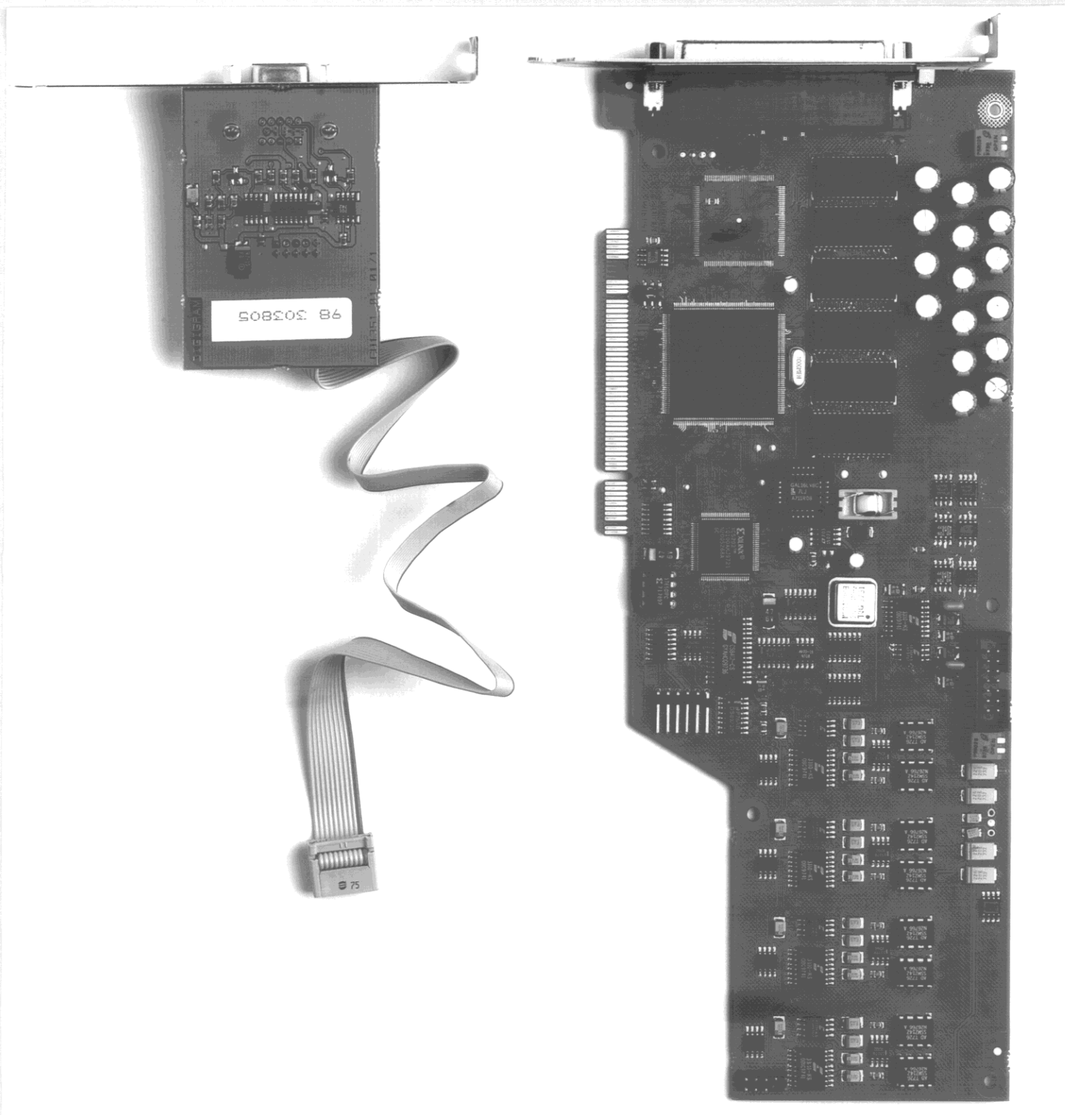
Figure 8.2..PCX820np and option Board, component side
