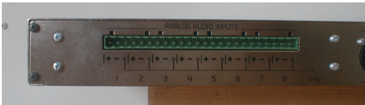
Detail view, rear side (ES8 OUT &IN – Terminal block connectors)
