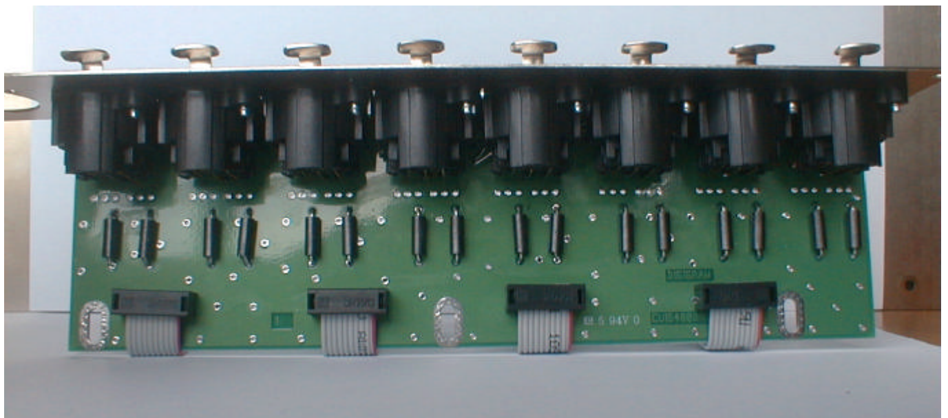
XLR connector board (ES8 IN &OUT)
