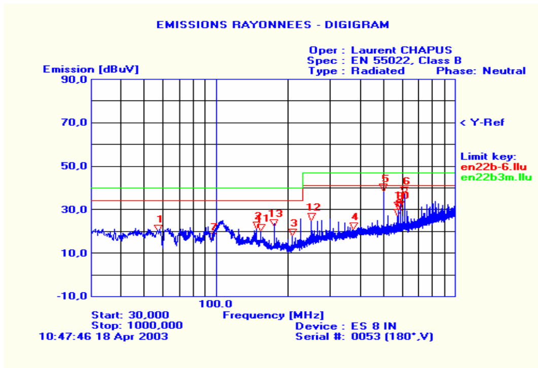
Graph [30MHz-1GHz] ES8 IN - XLR connectors
