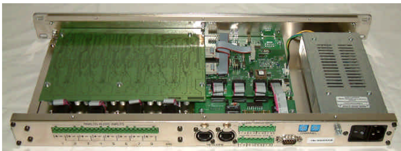
General view, cover removed, rear face (ES8mic- Terminal Block connectors)
