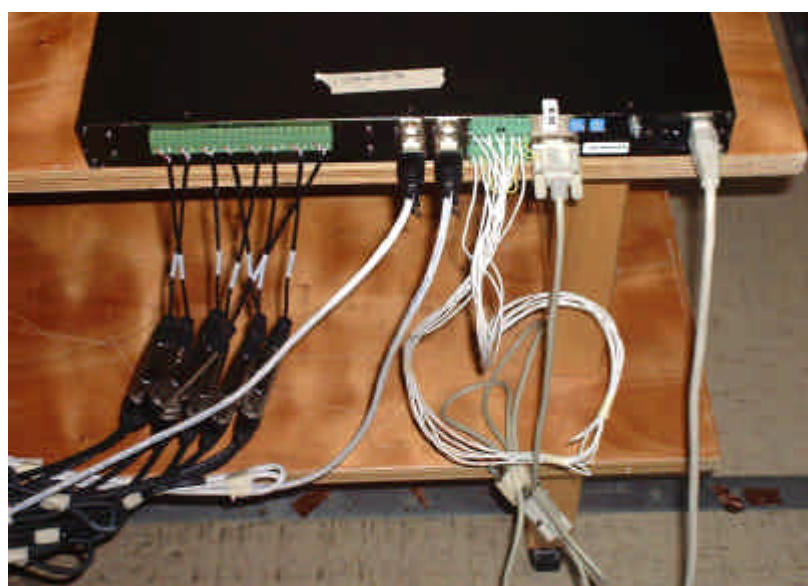
Detail view (Terminal Block connectors)
