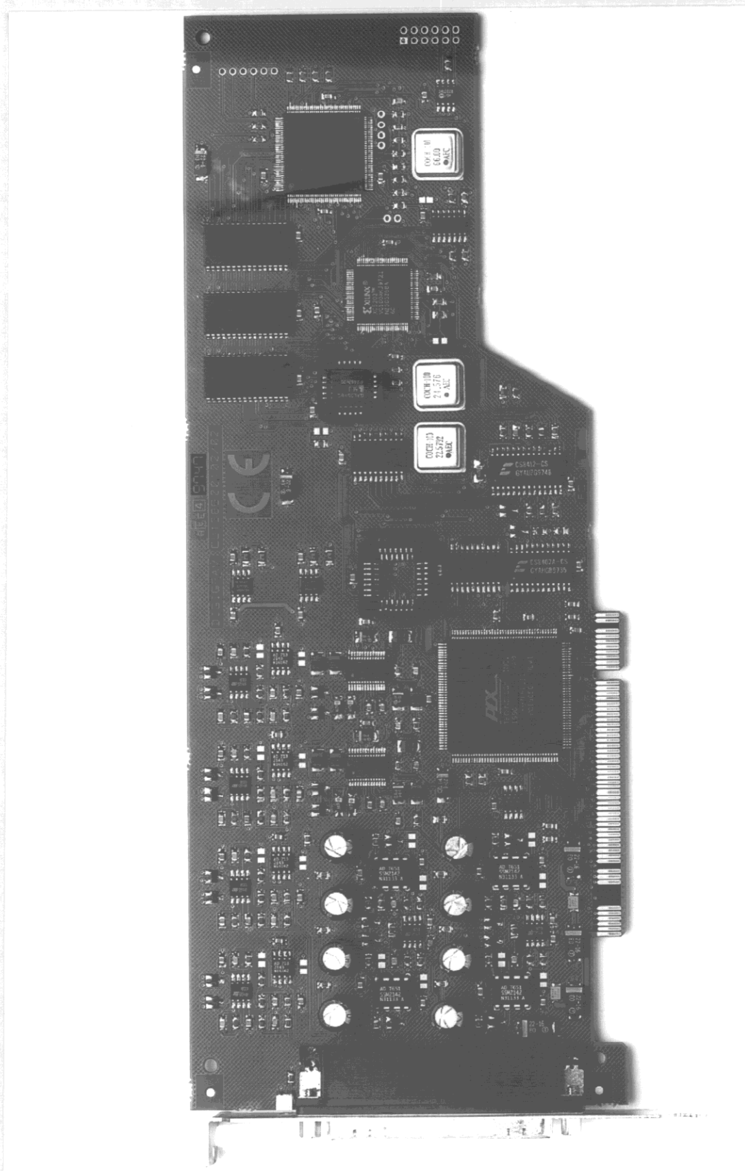
Figure 8.2..LCM 440 Board, component side
