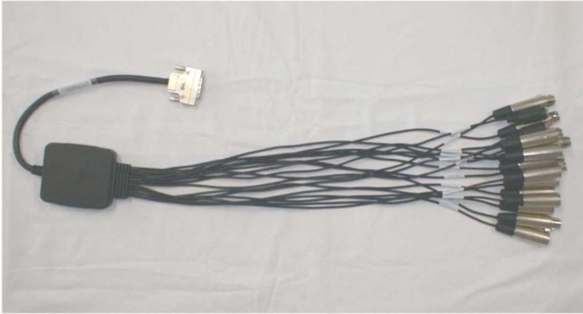
MiXart8 breakout cable for analog I/O (main card)
