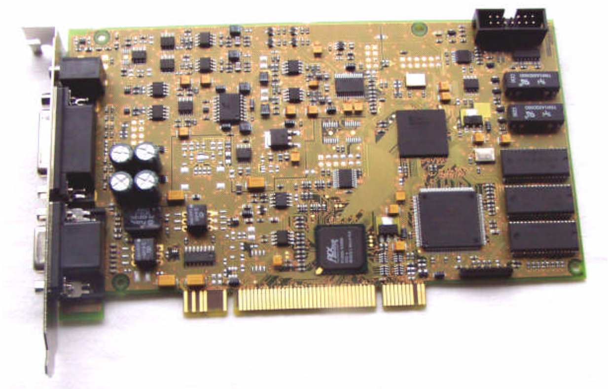
Components side
