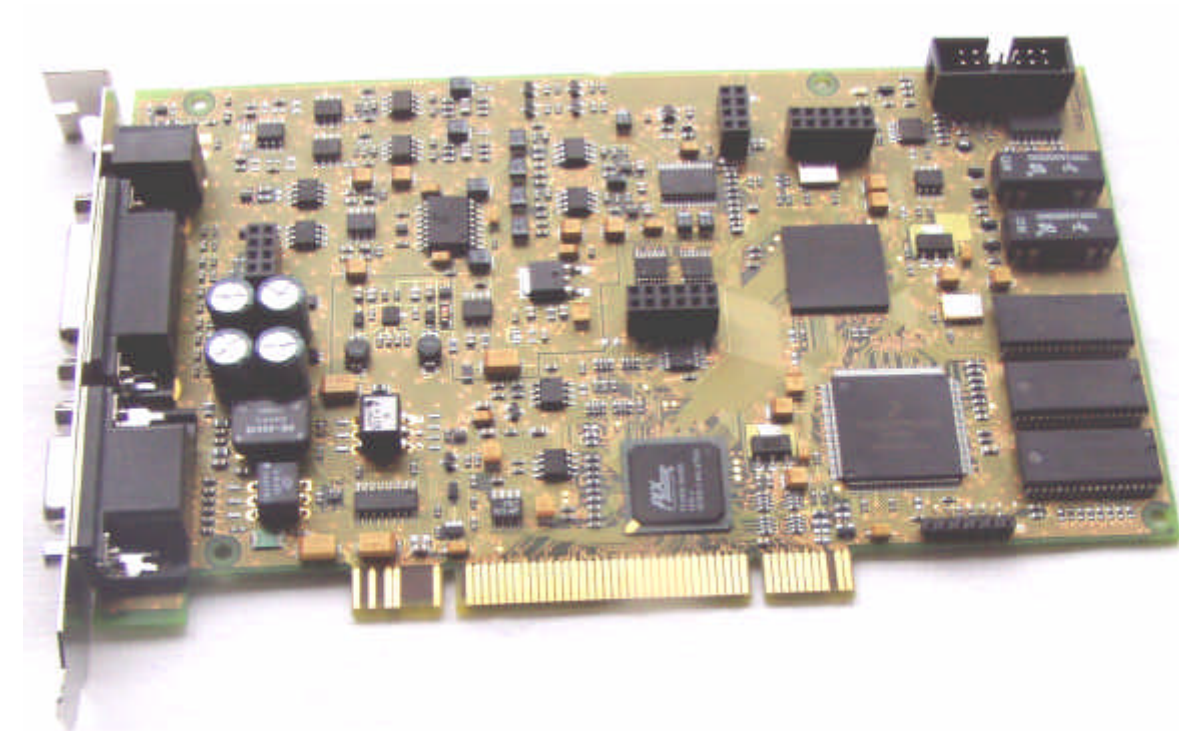
Components side without daughter board
