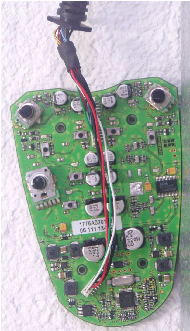
PCB views (UAX220-MIC & UAX220-v2)
