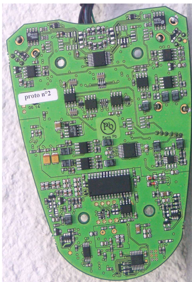
PCB views (UAX220-MIC & UAX220-v2)
