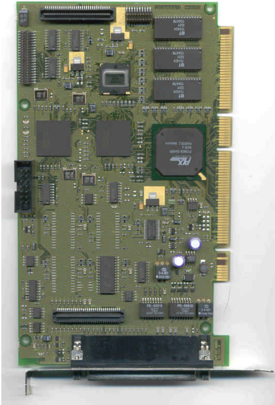
Components side
