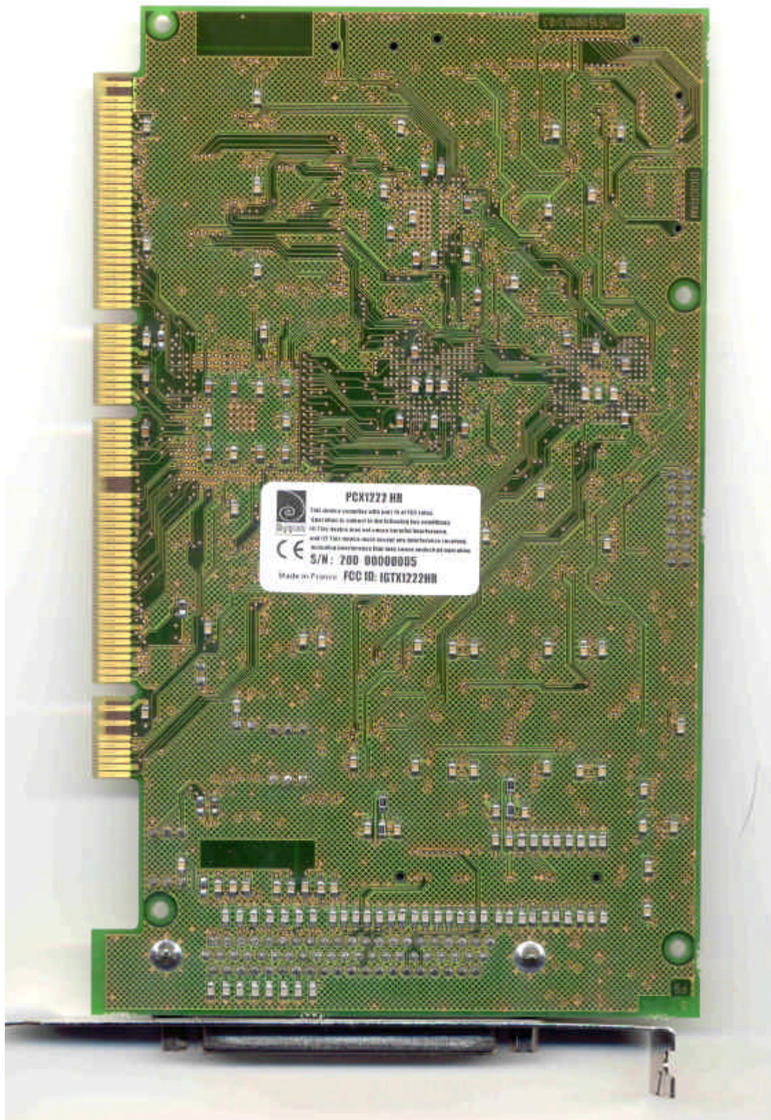
Solder side
