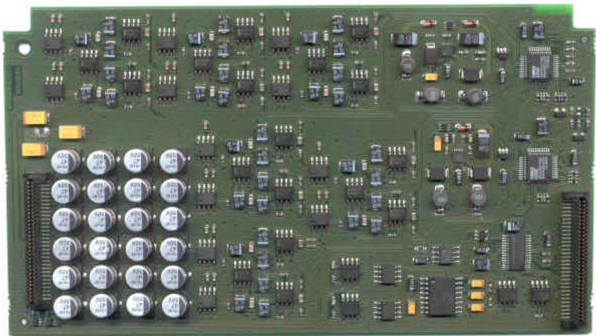
Components Side
