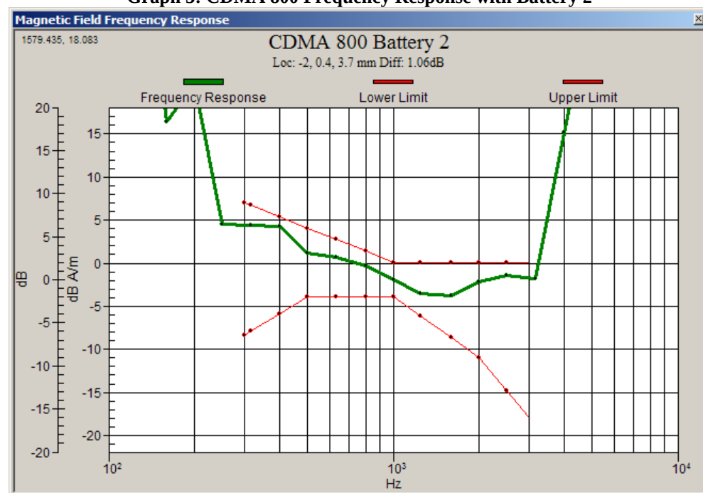
Graph 3: CDMA 800 Frequency Response with Battery 2
