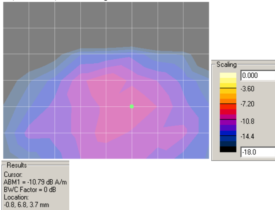
Y (Transverse) – ABM1 Signal
