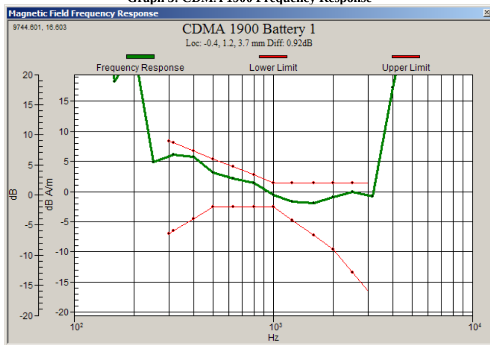
Graph 5: CDMA 1900 Frequency Response
