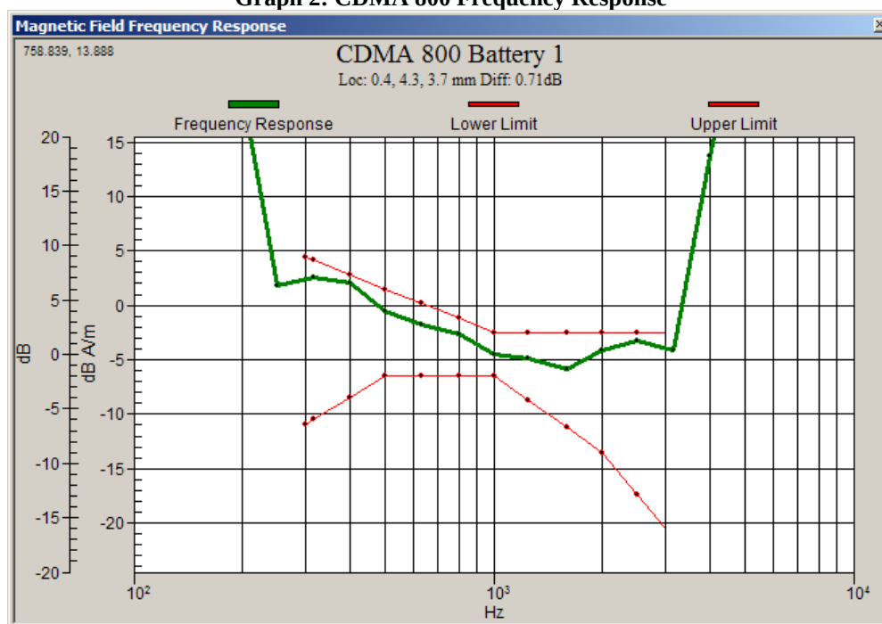
Graph 2: CDMA 800 Frequency Response
