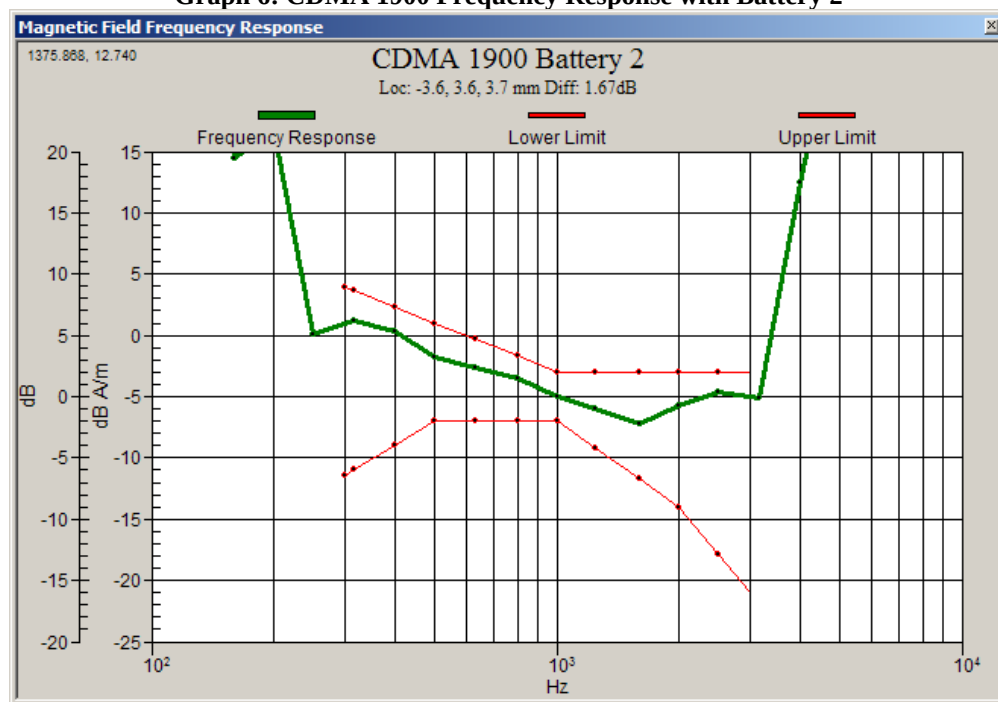
Graph 6: CDMA 1900 Frequency Response with Battery 2
