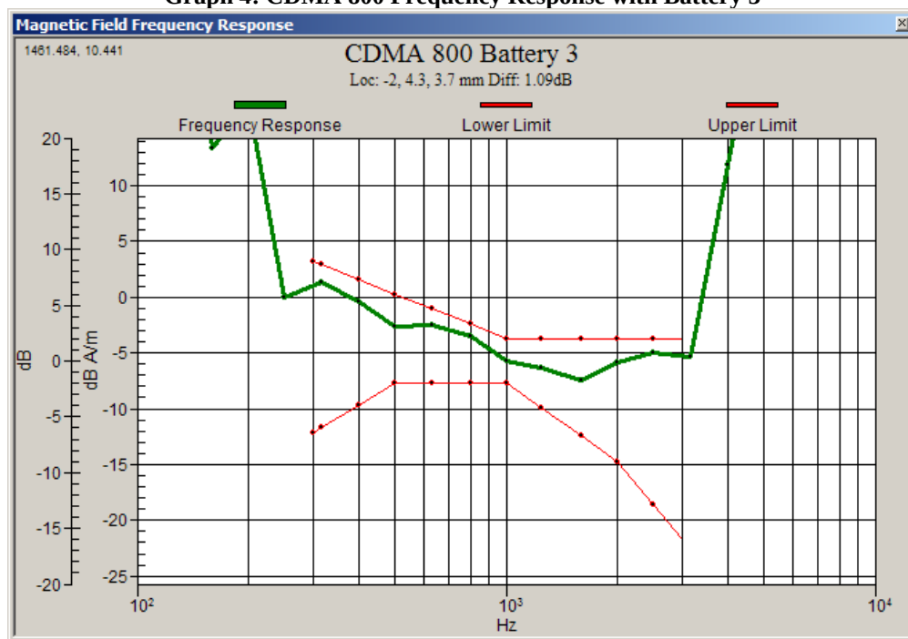
Graph 4: CDMA 800 Frequency Response with Battery 3
