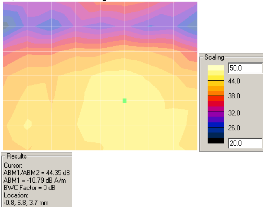
Y (Transverse) – ABM1 Signal
