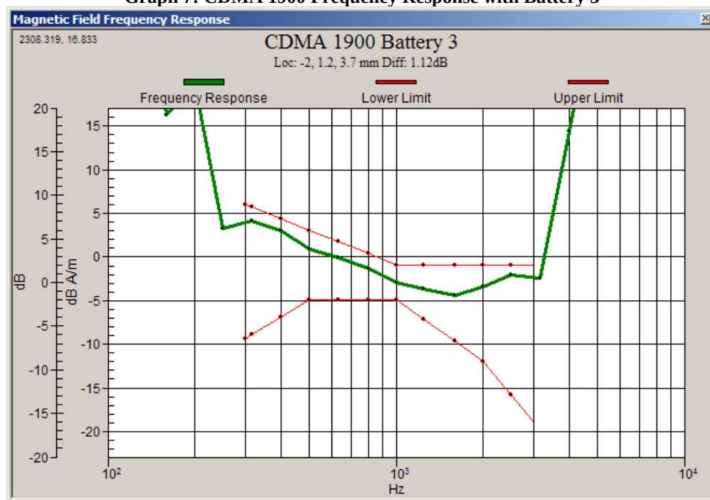
Graph 7: CDMA 1900 Frequency Response with Battery 3
