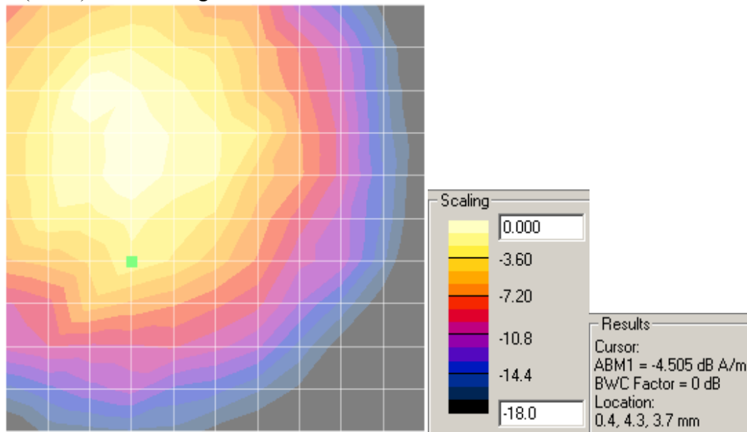
Z (Axial) – ABM1 Signal
