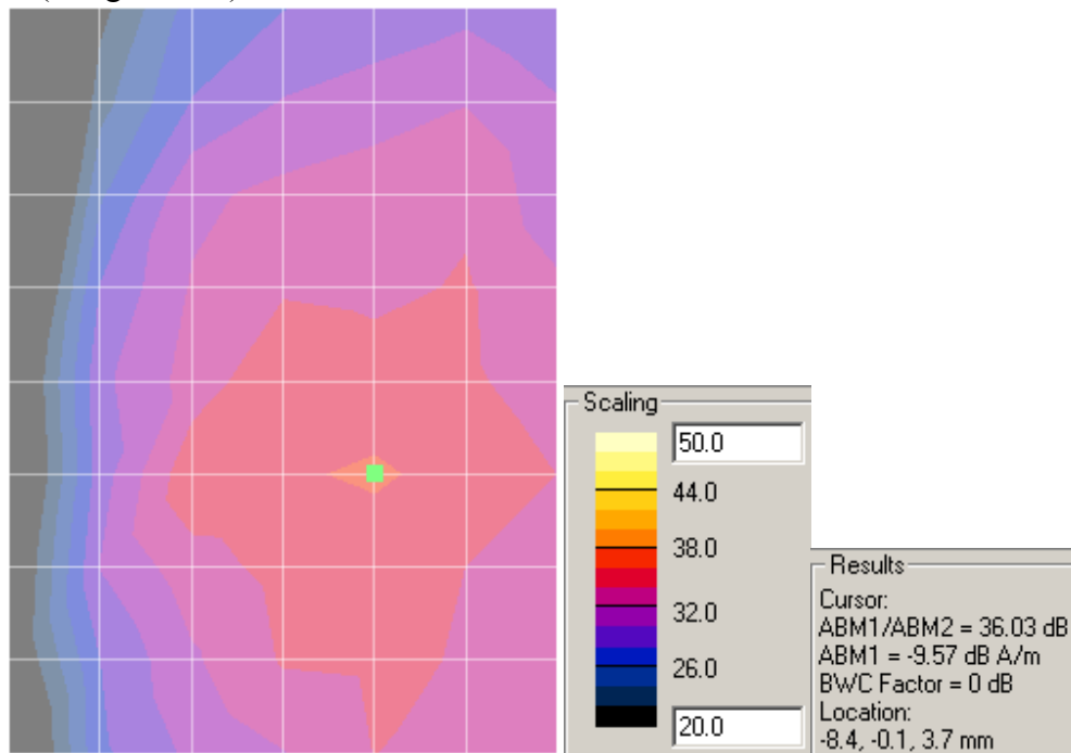
X (Longitudinal) – SNR
