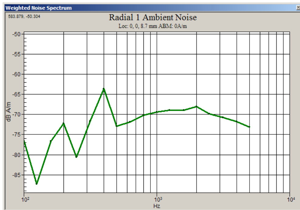
Graph A2-2. Radial 1 (Longitudinal) Position Ambient Noise Spectrum Plot
