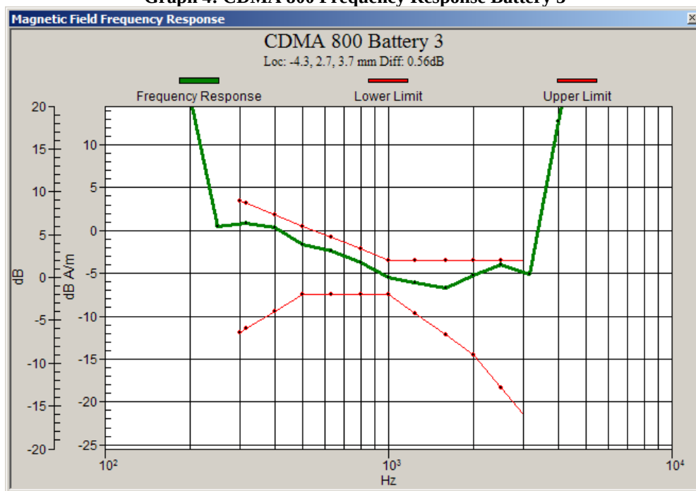
Graph 4: CDMA 800 Frequency Response Battery 3
