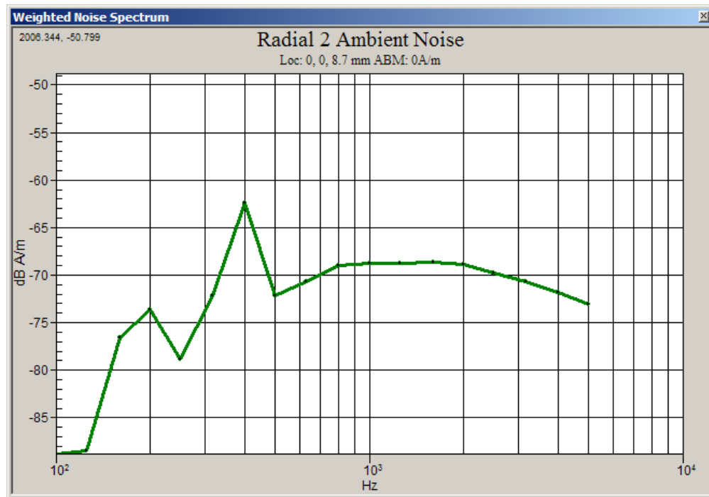
Graph A2-3. Radial 2 (Transverse) Position Ambient Noise Spectrum Plot
