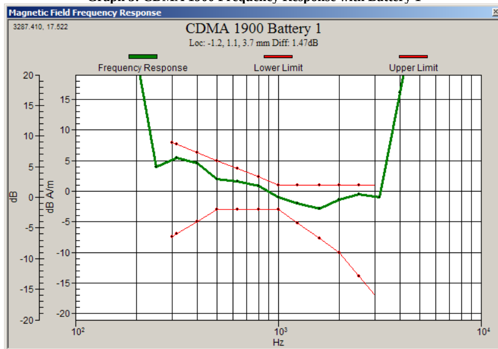
Graph 5: CDMA 1900 Frequency Response with Battery 1
