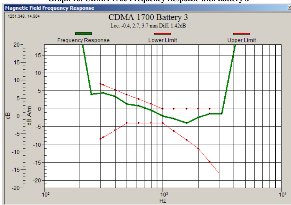
Graph 10: CDMA 1700 Frequency Response with Battery 3
