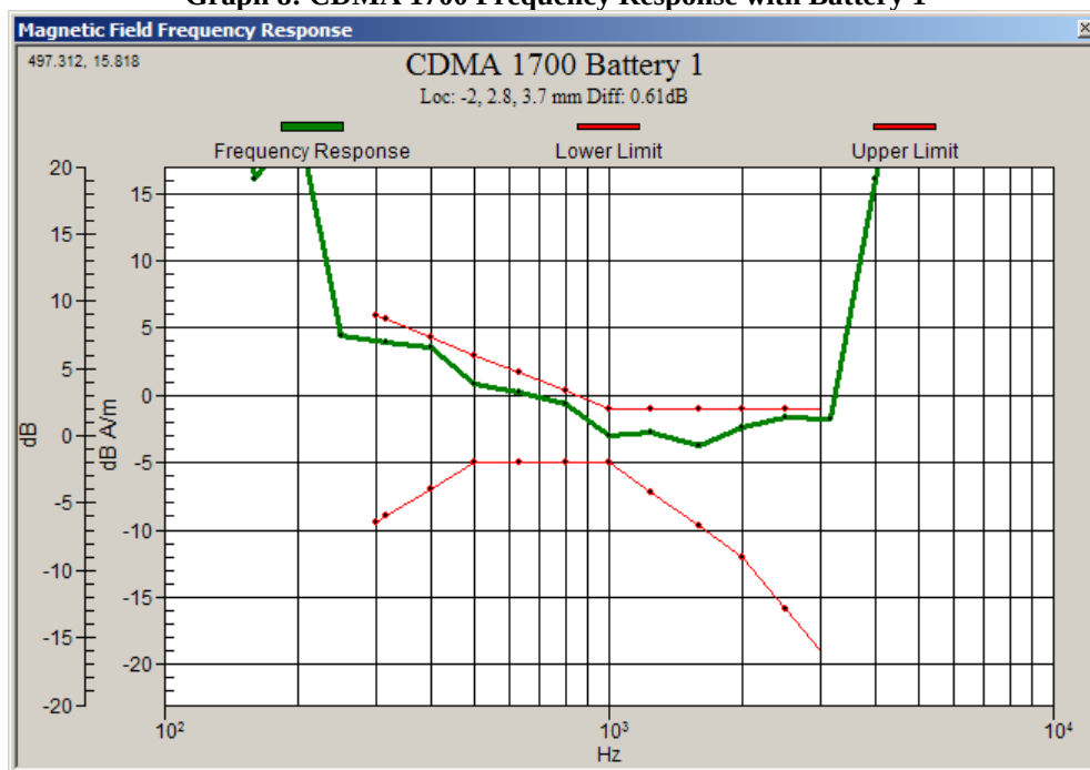
Graph 8: CDMA 1700 Frequency Response with Battery 1
