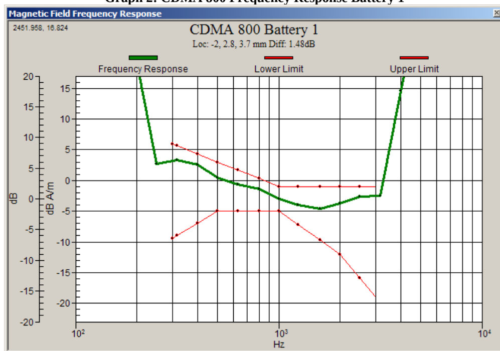
Graph 2: CDMA 800 Frequency Response Battery 1
