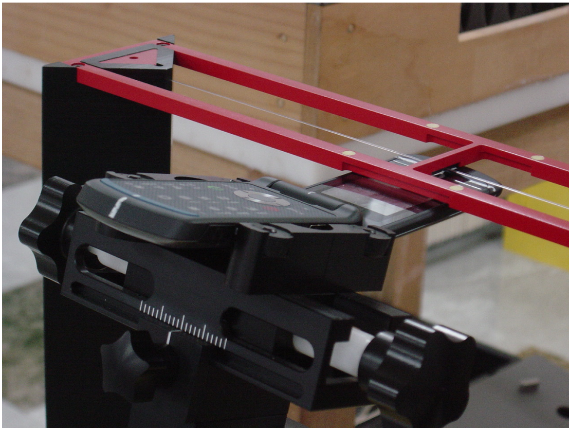
Figure 4. Positioning and Measurement for RF Emissions
