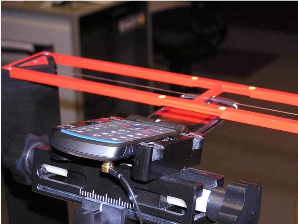
Figure 7. Positioning and Measurement for T-coil
